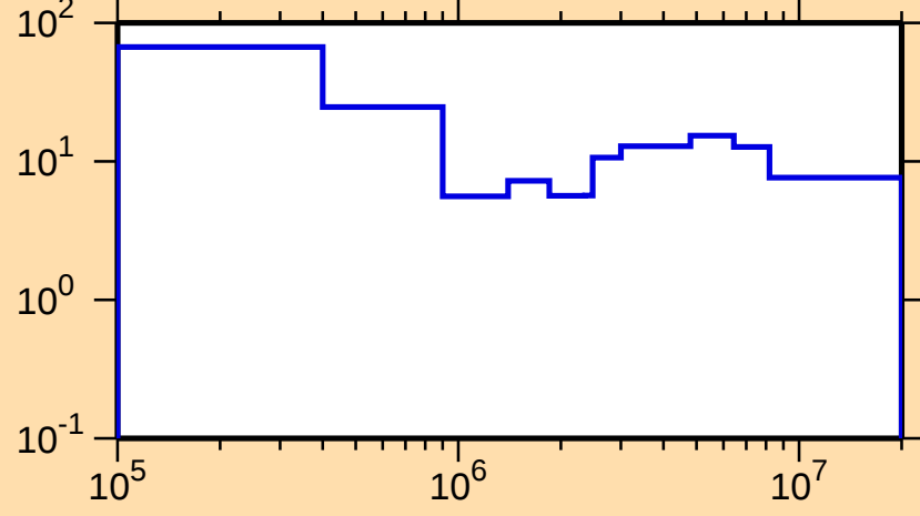
\Delta\sigma/\sigma vs. E for ^{144}\text{Ba}(\text{n,nonel.})
