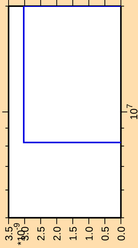
\Delta\sigma/\sigma vs. E for ^{144}\text{Ba}(\text{mt } 11)
