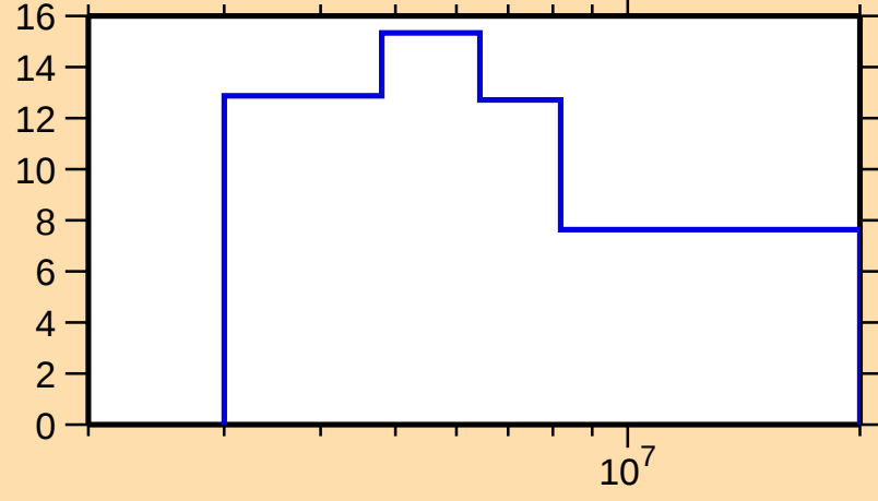
\Delta\sigma/\sigma vs. E for ^{144}\text{Ba}(n,\text{nonel.})
