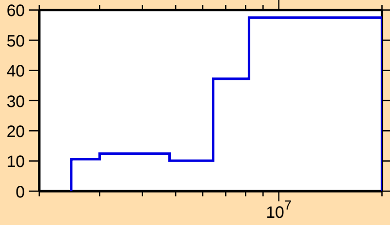
\Delta\sigma/\sigma vs. E for ^{144}\text{Ba}(\text{n},\text{inel.})
