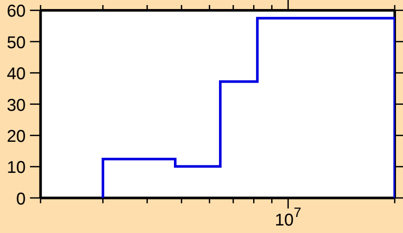
\Delta\sigma/\sigma vs. E for ^{144}\text{Ba}(n,\text{inel.})
