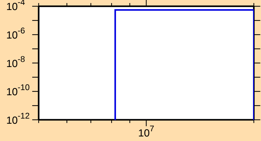
\sigma vs. E for ^{144}\text{Ba}(n,p)
