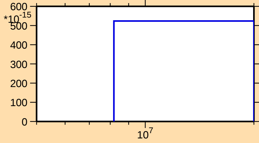
\sigma vs. E for ^{144}\text{Ba}(n,2np)
