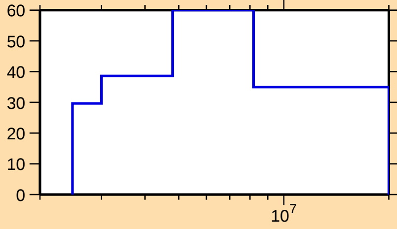
\Delta\sigma/\sigma vs. E for ^{144}\text{Ba}(\text{n},\text{el.})
