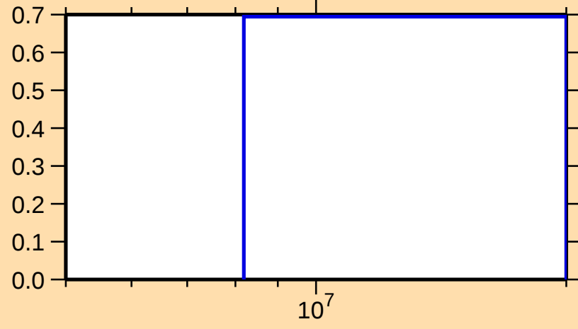
\sigma vs. E for ^{144}\text{Ba}(n,3n)
