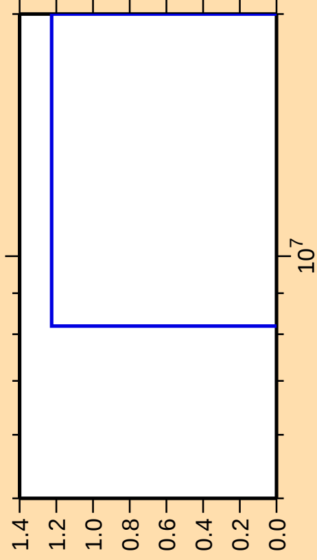
\Delta\sigma/\sigma vs. E for ^{144}\text{Ba}(n,2np)
