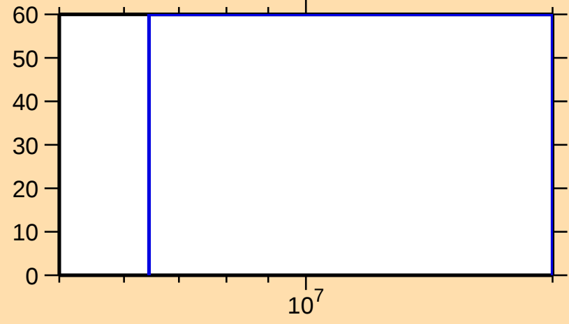
\Delta\sigma/\sigma vs. E for ^{144}\text{Ba}(n,n\text{cont.})
