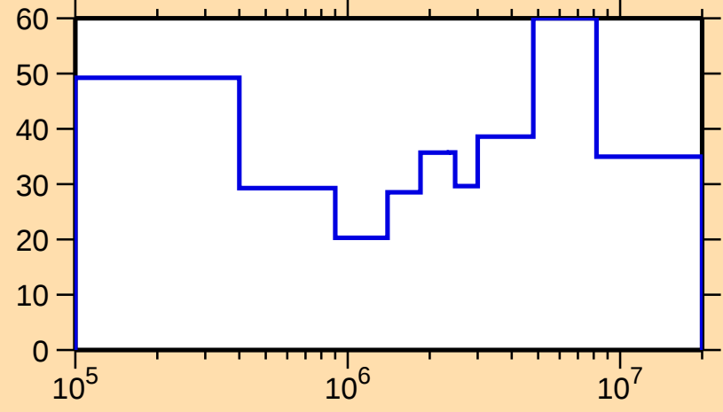
\Delta\sigma/\sigma vs. E for ^{144}\text{Ba}(n,\text{el.})
