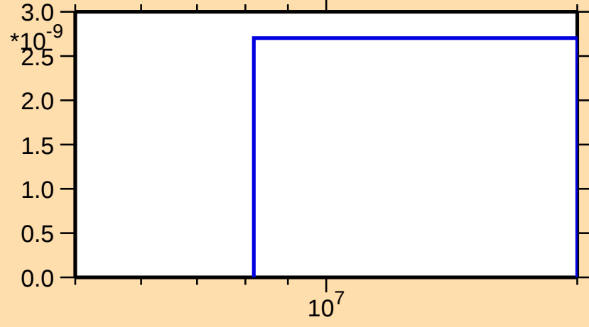
\sigma vs. E for ^{144}\text{Ba}(n,2n\alpha)
