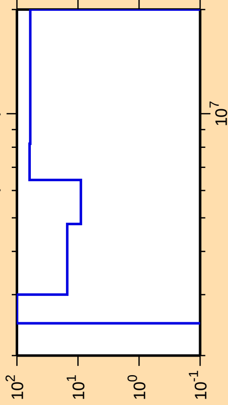
\Delta\sigma/\sigma vs. E for ^{144}\text{Ba}(n,\text{ncont.})
