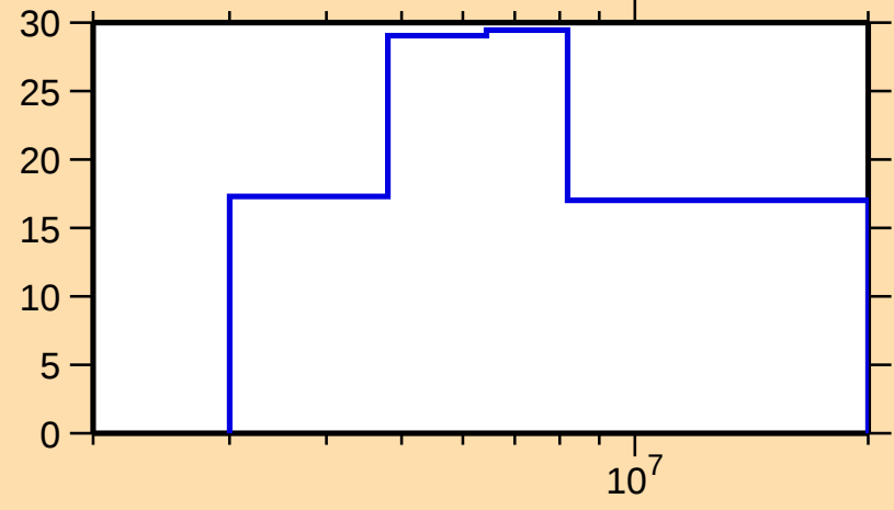
\Delta\sigma/\sigma vs. E for ^{144}\text{Ba}(n,\text{tot.})
