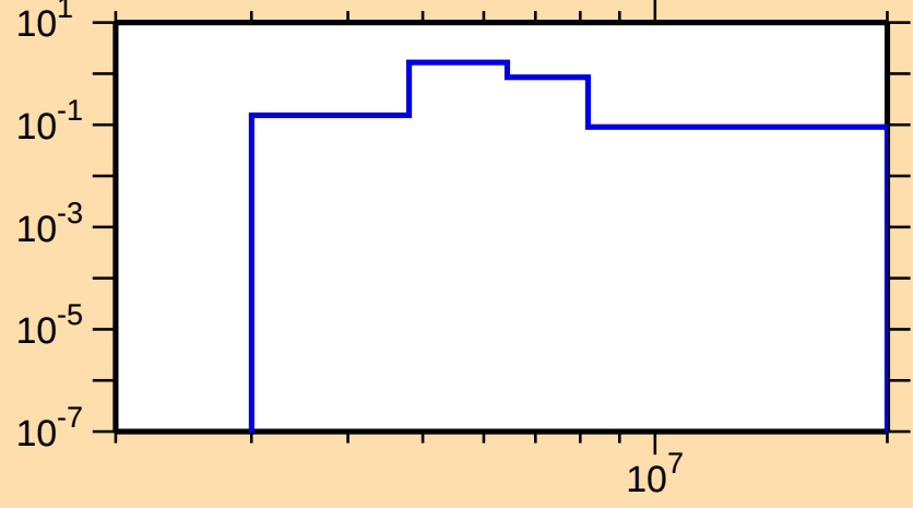
\sigma vs. E for ^{144}\text{Ba}(n,n\text{cont.})
