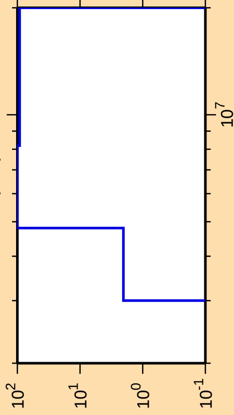
\Delta\sigma/\sigma vs. E for ^{144}\text{Ba}(n,\alpha)
