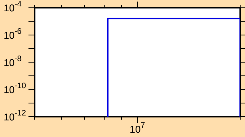
\sigma vs. E for ^{144}\text{Ba}(n,n\alpha)
