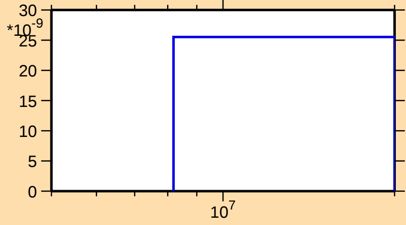
\sigma vs. E for ^{144}\text{Ba}(n,nt)
