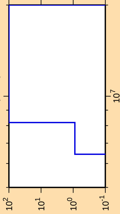
\Delta\sigma/\sigma vs. E for ^{144}\text{Ba}(n,n\alpha)
