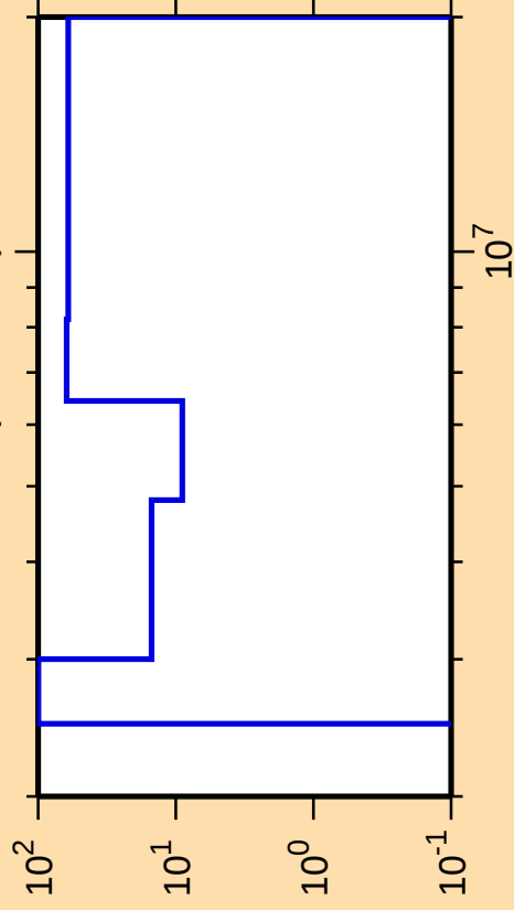
\Delta\sigma/\sigma vs. E for ^{144}\text{Ba}(n,n\text{cont.})
