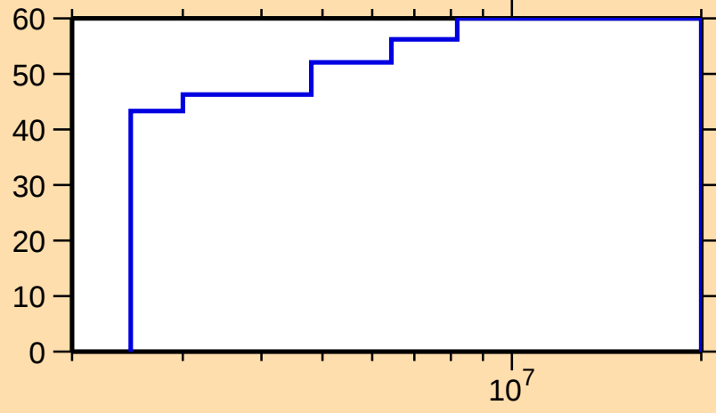
\Delta\sigma/\sigma vs. E for ^{144}\text{Ba}(n,n_1)
