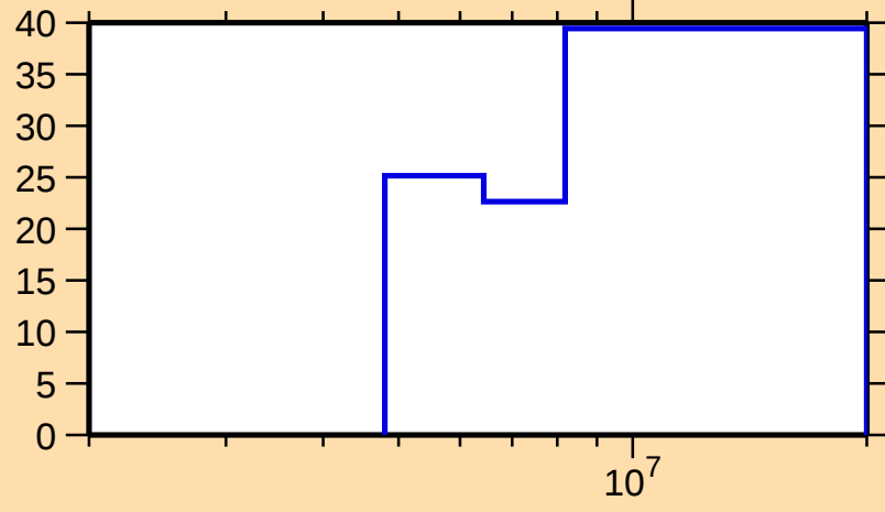
\Delta\sigma/\sigma vs. E for ^{144}\text{Ba}(n,2n)
