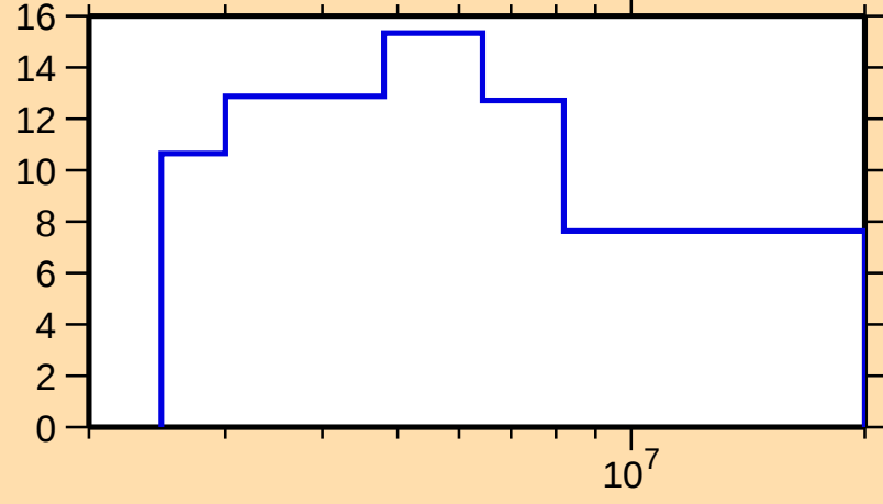
\Delta\sigma/\sigma vs. E for ^{144}\text{Ba}(\text{n},\text{nonel.})
