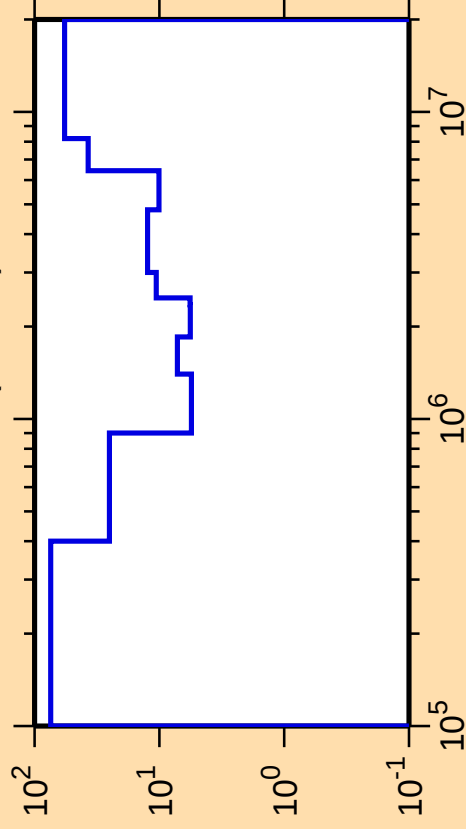
\Delta\sigma/\sigma vs. E for ^{144}\text{Ba}(n,\text{inel.})
