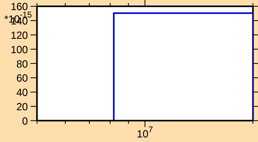
\sigma vs. E for ^{144}\text{Ba}(n,3n\alpha)
