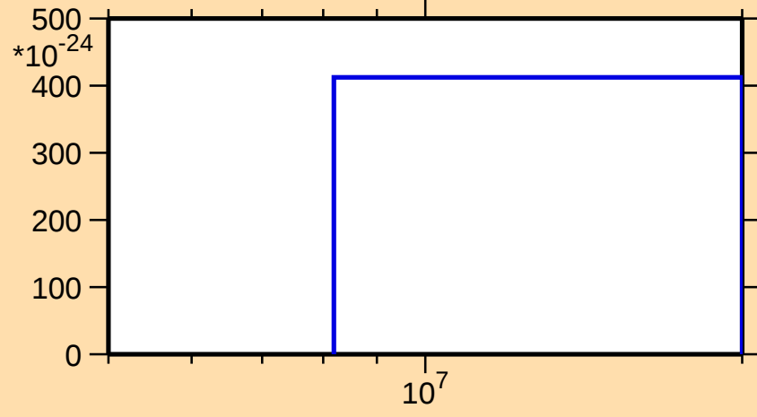
\sigma vs. E for ^{144}\text{Ba}(\text{mt } 11)
