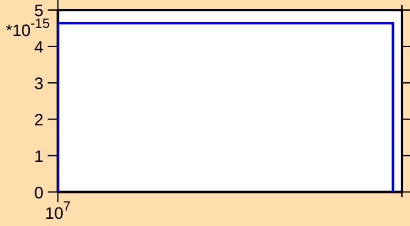
\sigma vs. E for ^{146}\text{Ba}(n,3n\alpha)
