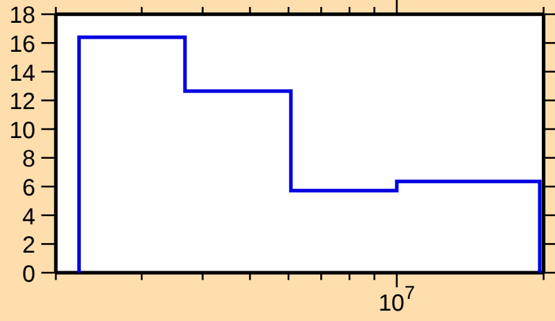
\Delta\sigma/\sigma vs. E for ^{146}\text{Ba}(n,\text{tot.})
