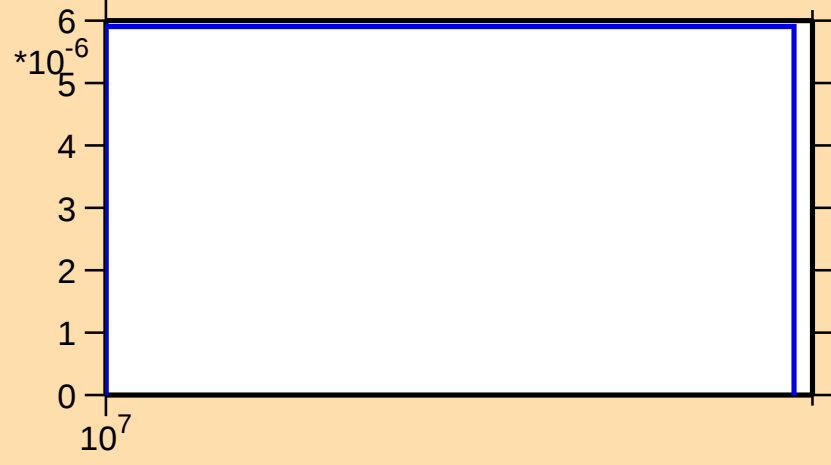
\sigma vs. E for ^{146}\text{Ba}(n,t)
