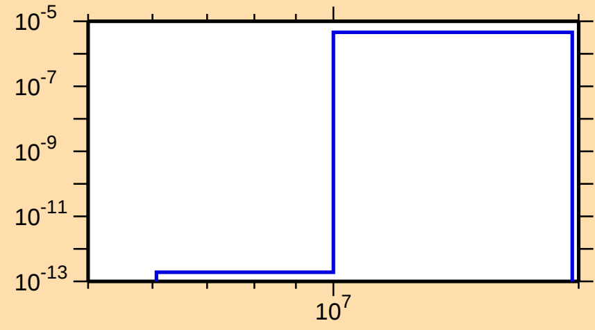
\sigma vs. E for ^{146}\text{Ba}(n,n\alpha)
