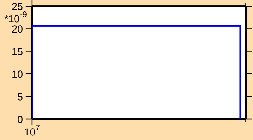
\sigma vs. E for ^{146}\text{Ba}(n,\text{nt})
