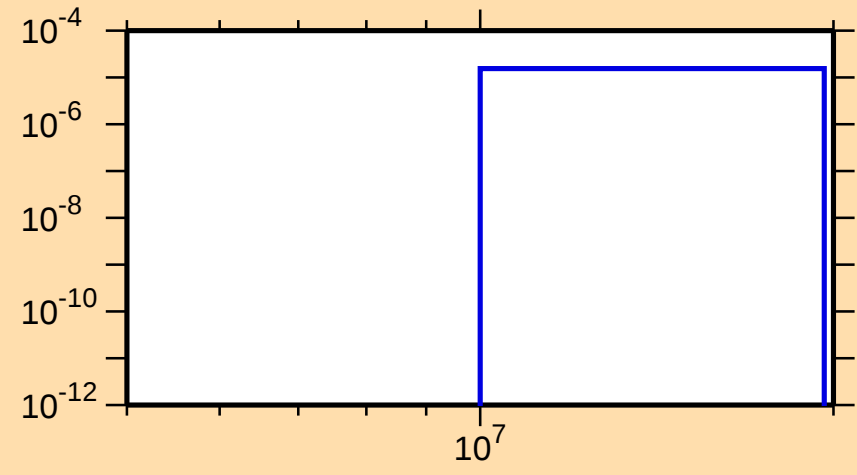
\sigma vs. E for ^{146}\text{Ba}(n,p)
