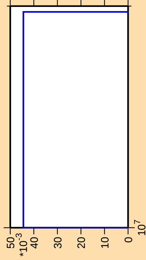
\Delta\sigma/\sigma vs. E for ^{146}\text{Ba}(n,2np)
