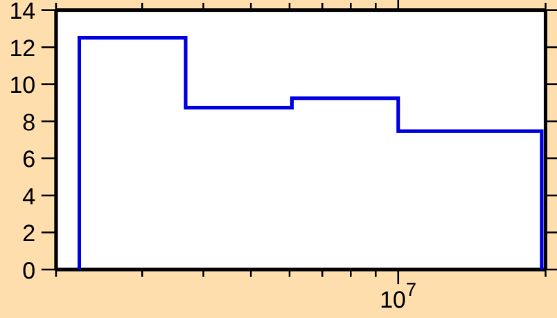
\Delta\sigma/\sigma vs. E for ^{146}\text{Ba}(n,n\text{onel.})
