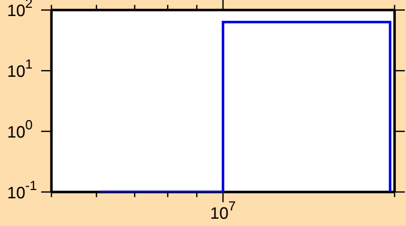
\Delta\sigma/\sigma vs. E for ^{146}\text{Ba}(n,p)
