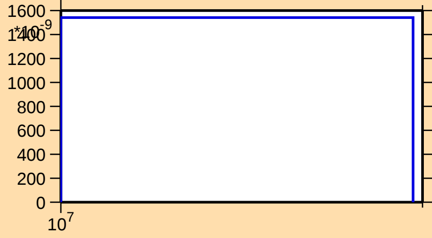
\sigma vs. E for ^{146}\text{Ba}(n,d)
