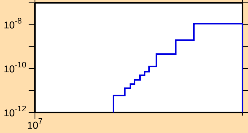
\sigma vs. E for ^{270}\text{He3} )
