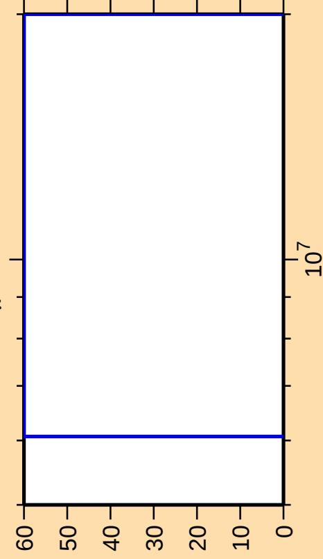
\Delta\sigma/\sigma vs. E for ^{271}\gamma
