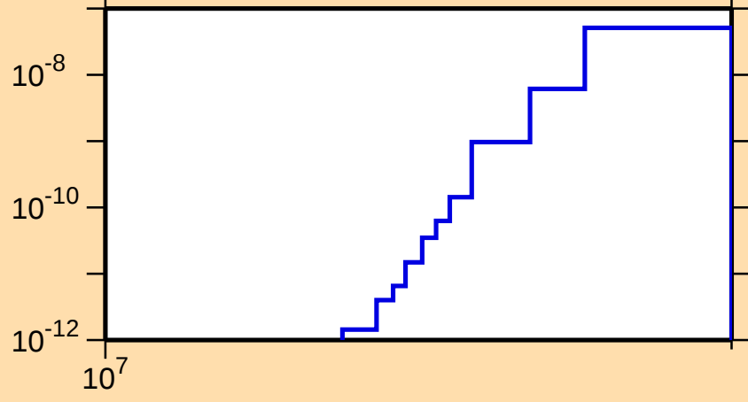
\sigma vs. E for ^{271}
