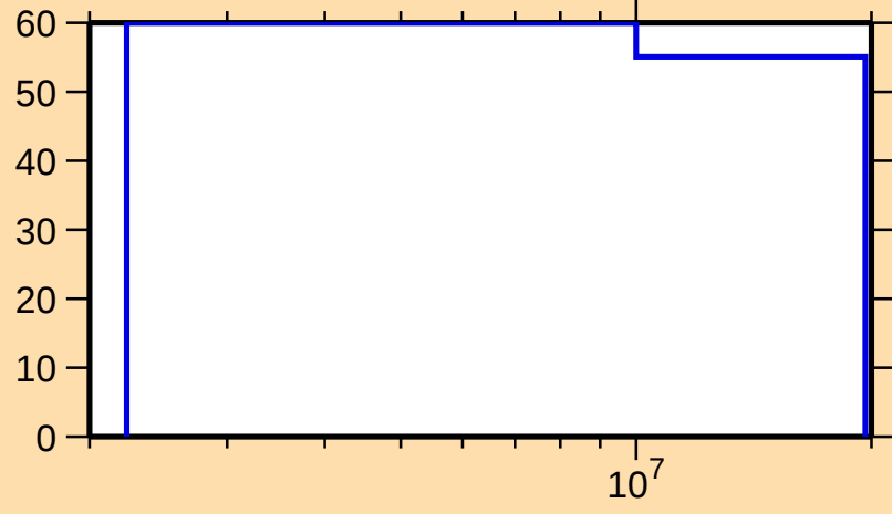
\Delta\sigma/\sigma vs. E for ^{271}\text{Lu}
