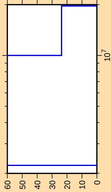
\Delta\sigma/\sigma vs. E for ^{271}\text{Lu}
