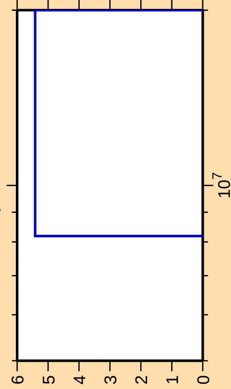
\Delta\sigma/\sigma vs. E for ^{271}\alpha )
