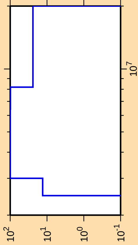
\Delta\sigma/\sigma vs. E for ^{271}\text{Po}
