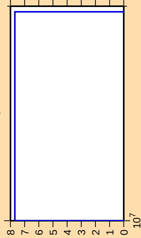
\Delta\sigma/\sigma vs. E for ^{272}\text{He3} )
