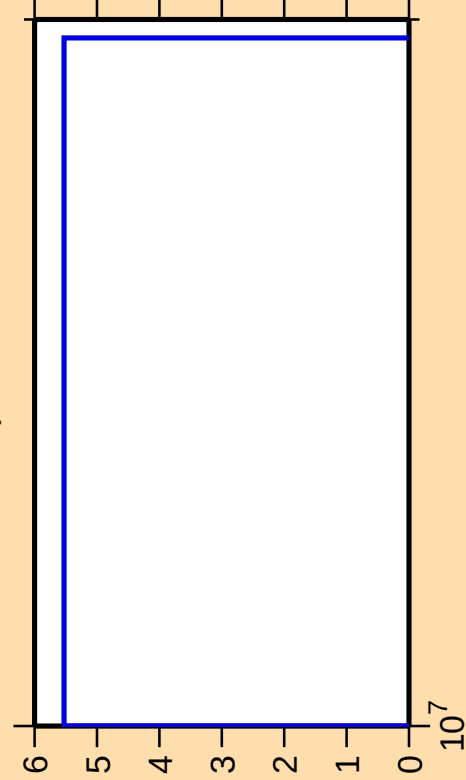
\Delta\sigma/\sigma vs. E for ^{272}\alpha )
