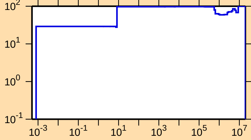
\Delta\sigma/\sigma vs. E for ^{275}\gamma )
