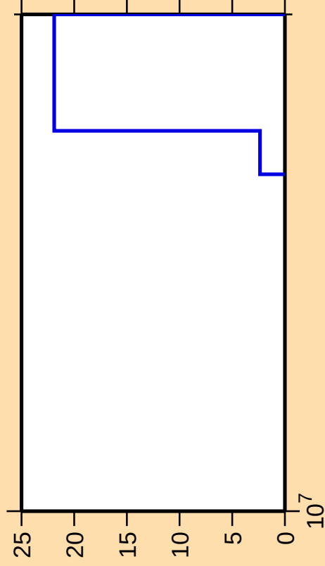
\Delta\sigma/\sigma vs. E for ^{275}\alpha )
