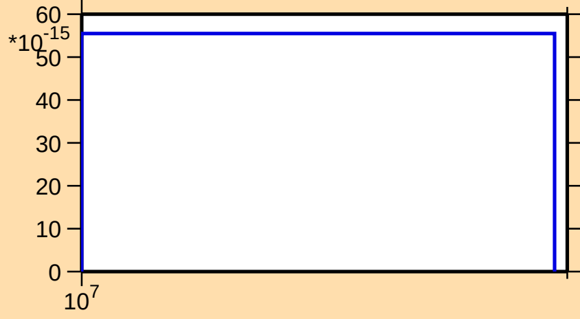
\sigma vs. E for ^{275}\alpha )
