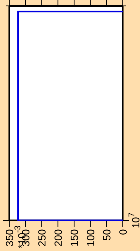
\Delta\sigma/\sigma vs. E for ^{275}\alpha )
