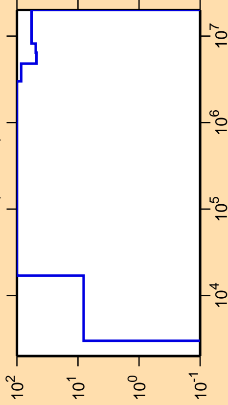
\Delta\sigma/\sigma vs. E for ^{190}\text{Bi}(n,\text{inel.})
