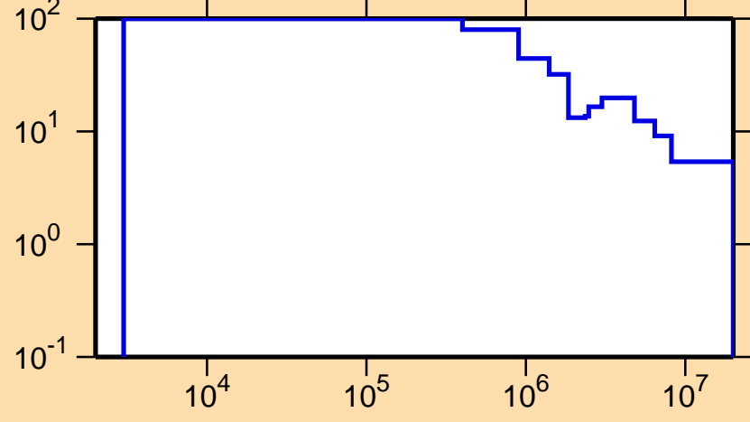
\Delta\sigma/\sigma vs. E for ^{190}\text{Bi}(n,n\text{onel.})
