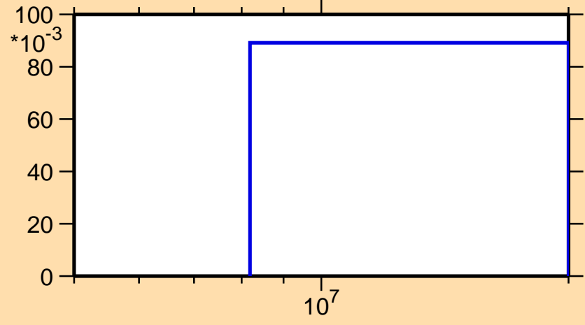
\sigma vs. E for ^{190}\text{Bi}(n,2n)
