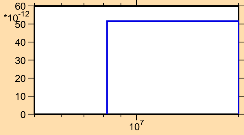
\sigma vs. E for ^{190}\text{Bi}(n,\text{nt})
