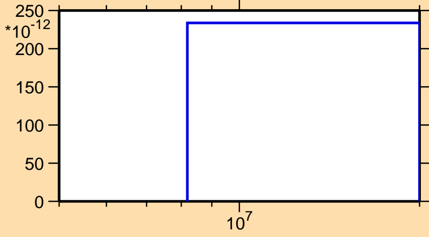
\sigma vs. E for ^{190}\text{Bi}(\text{mt } 34)
