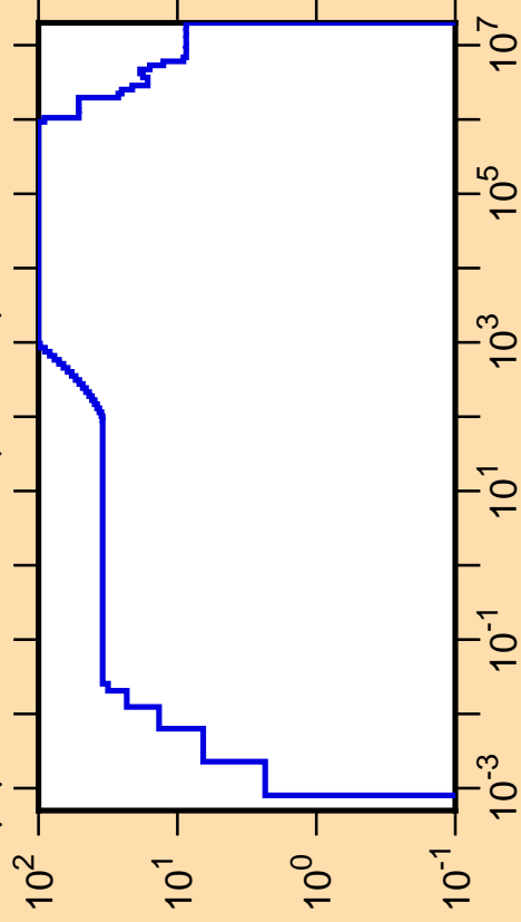
\Delta\mu/\mu vs. E for ^{192}\text{Bi}(\text{mt251})
