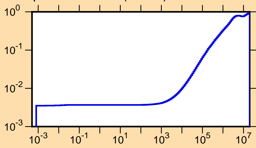
\mu vs. E for ^{192}\text{Bi}(\text{mt251})
