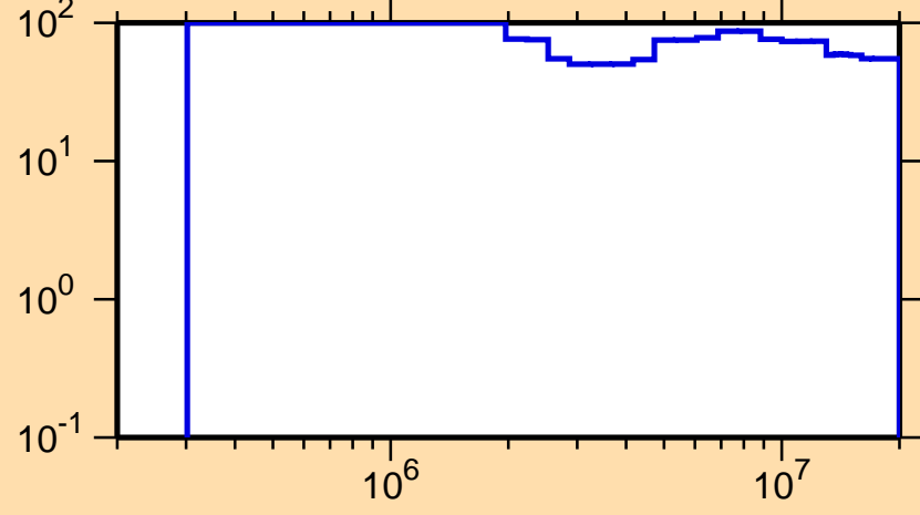
\Delta\sigma/\sigma vs. E for ^{193}\text{Bi}(n,n_1)
