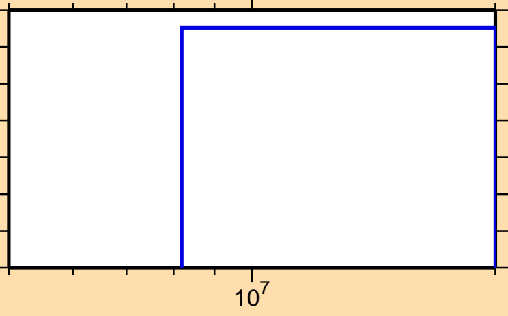
\sigma vs. E for ^{193}\text{Bi}(n,3n)
