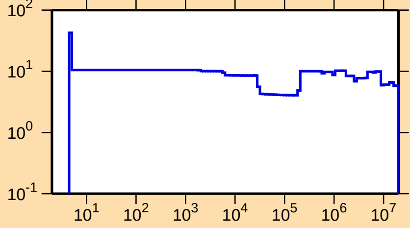
\Delta\sigma/\sigma vs. E for ^{194}\text{Bi}(n,\text{el.})
