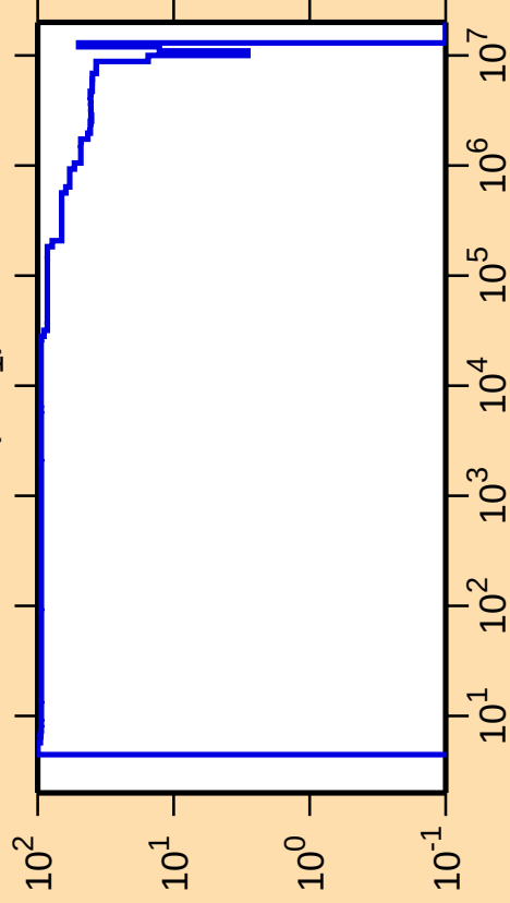
\Delta\sigma/\sigma vs. E for ^{194}\text{Bi}(n,n_1)
