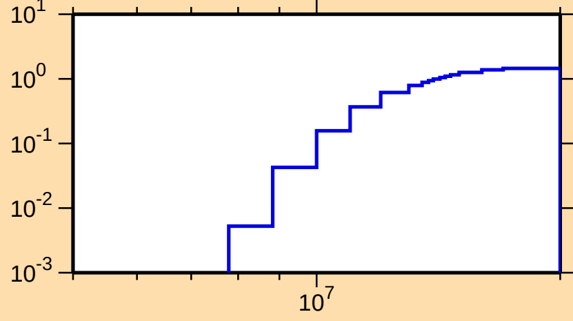
\sigma vs. E for ^{194}\text{Bi}(n,2n)
