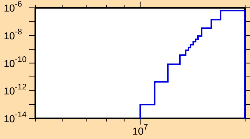
\sigma vs. E for ^{194}\text{Bi}(n,\text{pd})
