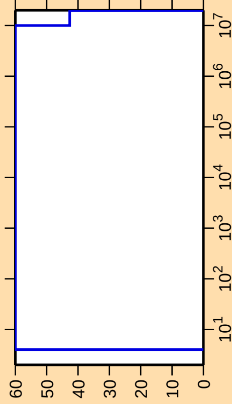
\Delta\sigma/\sigma vs. E for ^{194}\text{Bi}(n,p)
