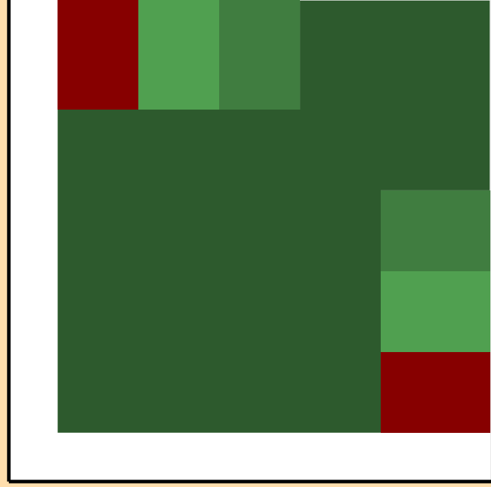
\sigma vs. E for ^{194}\text{Bi}(n,np)
