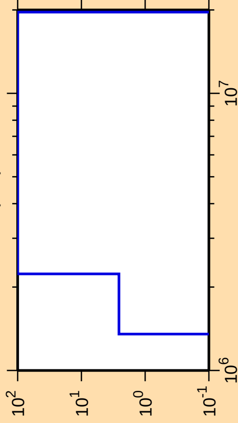
\Delta\sigma/\sigma vs. E for ^{194}\text{Bi}(n,d)
