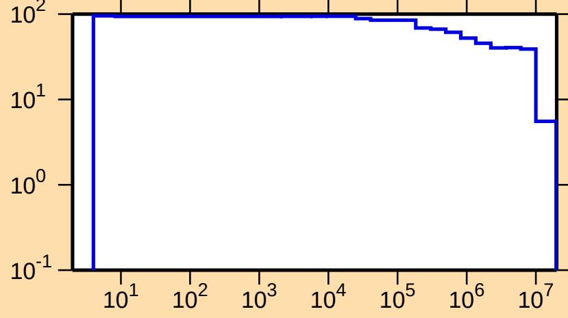
\Delta\sigma/\sigma vs. E for ^{194}\text{Bi}(n,n_1)
