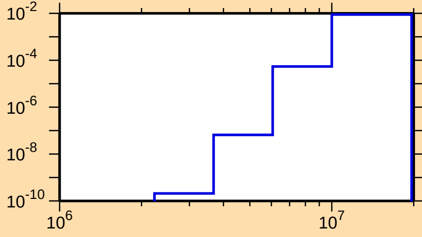
\sigma vs. E for ^{194}\text{Bi}(n,d)
