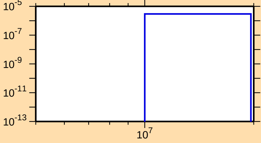
\sigma vs. E for ^{194}\text{Bi}(n,\text{nd})
