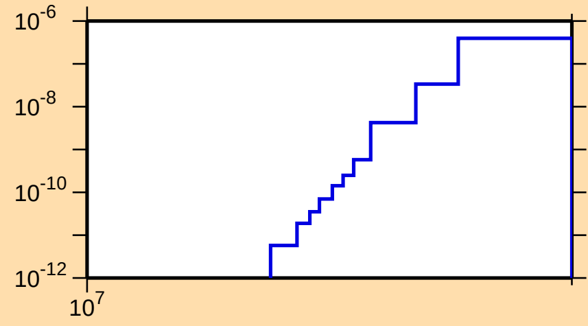
\sigma vs. E for ^{197}\text{Bi}(n,2n\alpha)
