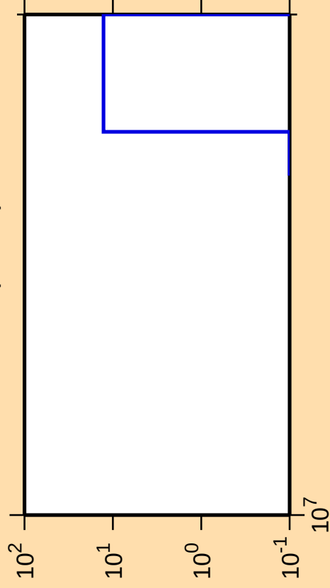
\Delta\sigma/\sigma vs. E for ^{197}\text{Bi}(\text{mt } 34)
