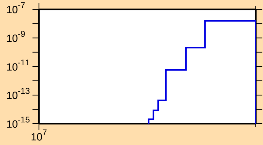
\sigma vs. E for ^{197}\text{Bi}(n,\text{nt})
