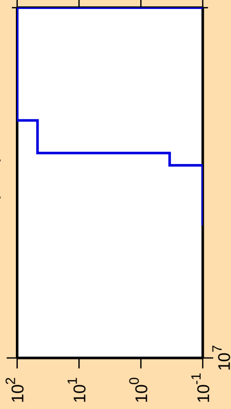
\Delta\sigma/\sigma vs. E for ^{197}\text{Bi}(n,\text{nt})
