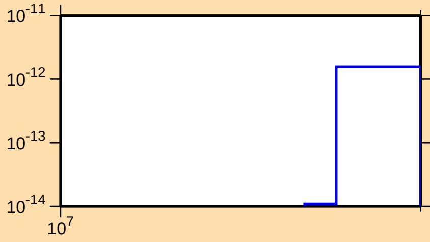
\sigma vs. E for ^{197}\text{Bi}(\text{mt } 34)
