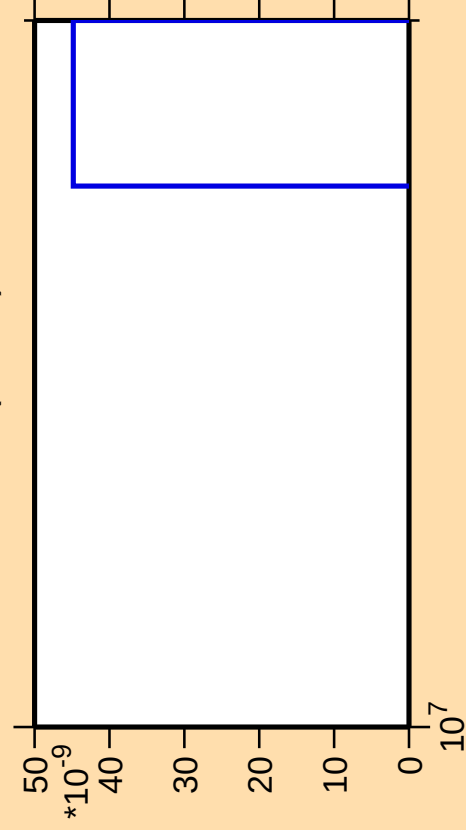
\Delta\sigma/\sigma vs. E for ^{197}\text{Bi} (mt 42)
