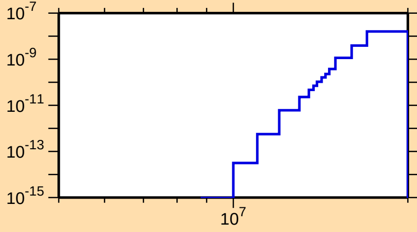
\sigma vs. E for ^{197}\text{Bi}(\text{mt } 45)
