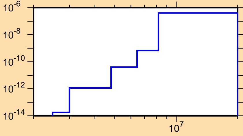
\sigma vs. E for ^{197}\text{Bi}(n,p\alpha)
