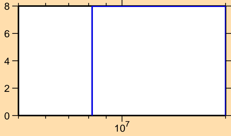
\Delta\sigma/\sigma vs. E for ^{197}\text{Bi}(n,\text{el.})
