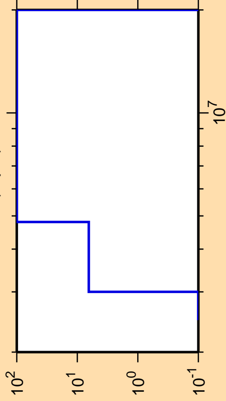
\Delta\sigma/\sigma vs. E for ^{197}\text{Bi}(n,p\alpha)
