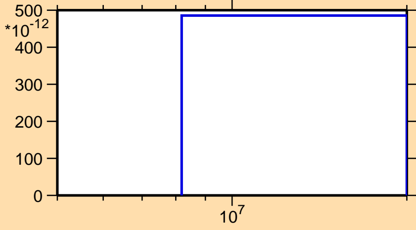
\sigma vs. E for ^{197}\text{Bi} (mt 45)
