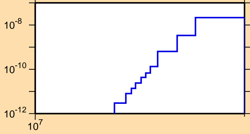
\sigma vs. E for ^{197}\text{Bi}(n,pd)
