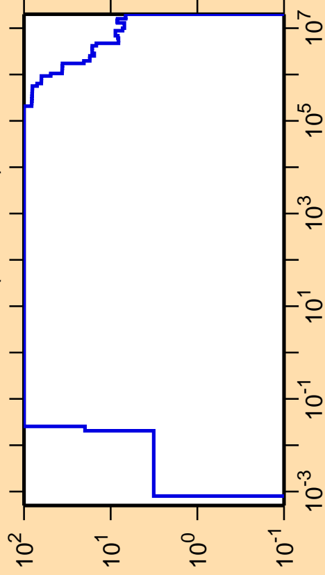
\Delta\sigma/\sigma vs. E for ^{197}\text{Bi}(n,\text{nonel.})
