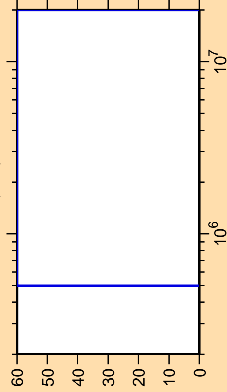
\Delta\sigma/\sigma vs. E for ^{197}\text{Bi}(n,\alpha)
