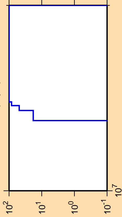
\Delta\sigma/\sigma vs. E for ^{197}\text{Bi}(n,pd)
