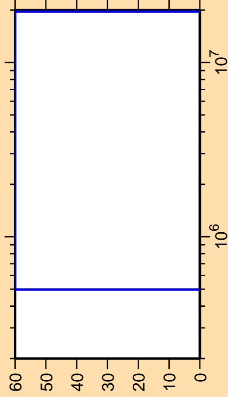
\Delta\sigma/\sigma vs. E for ^{197}\text{Bi}(n,p)
