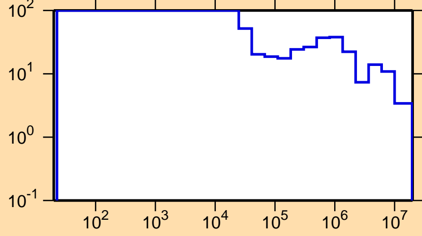
\Delta\sigma/\sigma vs. E for ^{197}\text{Bi}(n,\text{tot.})
