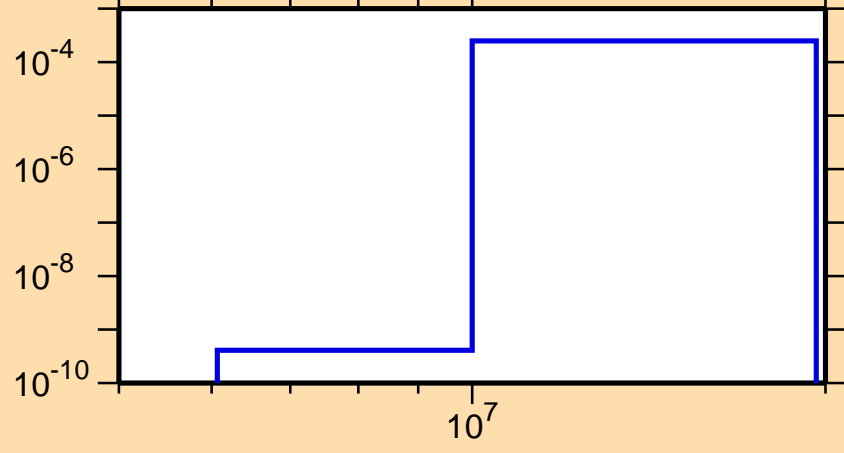
\sigma vs. E for ^{197}\text{Bi}(n,t)
