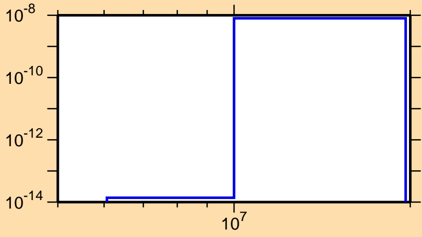
\sigma vs. E for ^{197}\text{Bi} (mt 45)
