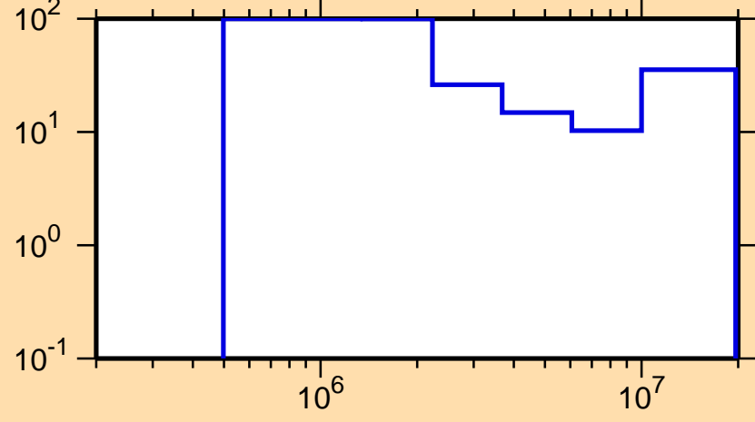
\Delta\sigma/\sigma vs. E for ^{197}\text{Bi}(n,n\text{cont.})
