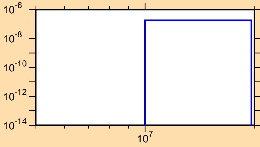
\sigma vs. E for ^{197}\text{Bi}(n,\text{nd})
