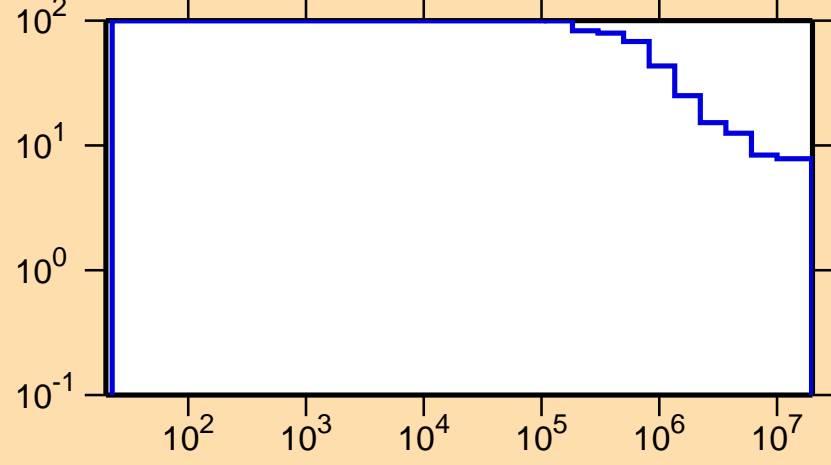
\Delta\sigma/\sigma vs. E for ^{197}\text{Bi}(n,\text{nonel.})
