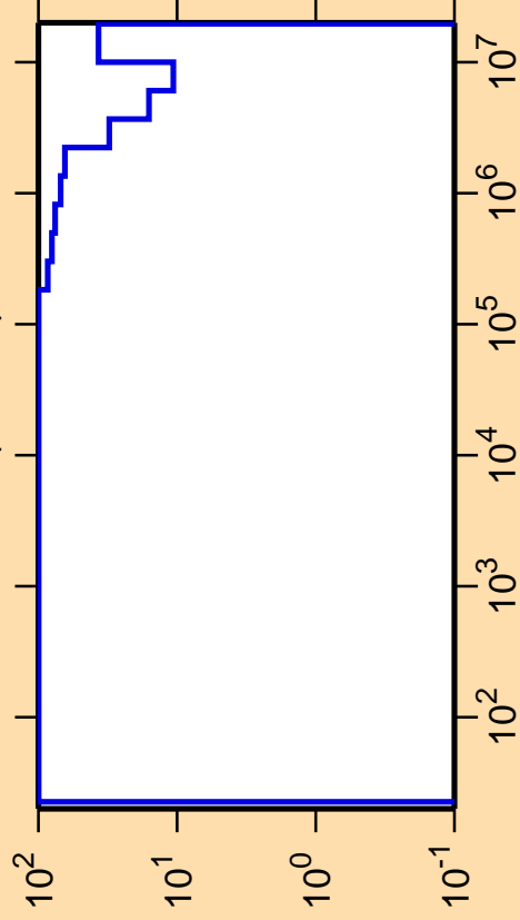
\Delta\sigma/\sigma vs. E for ^{197}\text{Bi}(n,\text{inel.})
