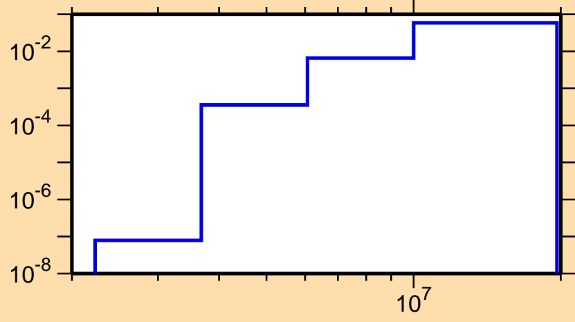
\sigma vs. E for ^{197}\text{Bi}(n,np)
