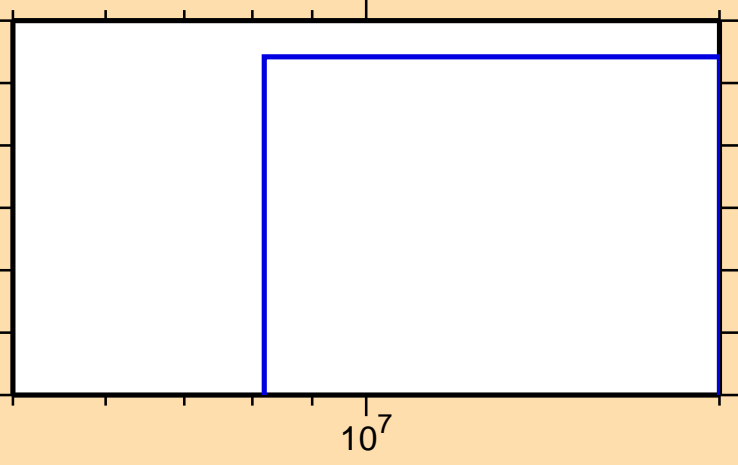
\sigma vs. E for ^{197}\text{Bi} (mt 42)
