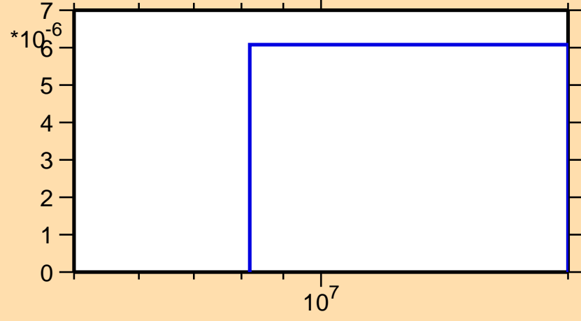
\sigma vs. E for ^{197}\text{Bi}(n,3n)
