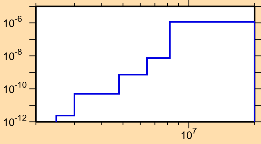
\sigma vs. E for ^{197}\text{Bi}(n,p\alpha)
