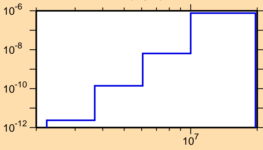
\sigma vs. E for ^{198}\text{Bi}(n,p\alpha)
