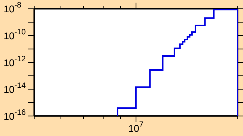
\sigma vs. E for ^{198}\text{Bi}(\text{mt } 45)
