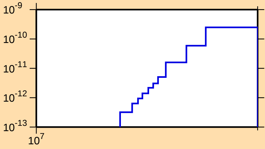
\sigma vs. E for ^{198}\text{Bi}(\text{mt117})
