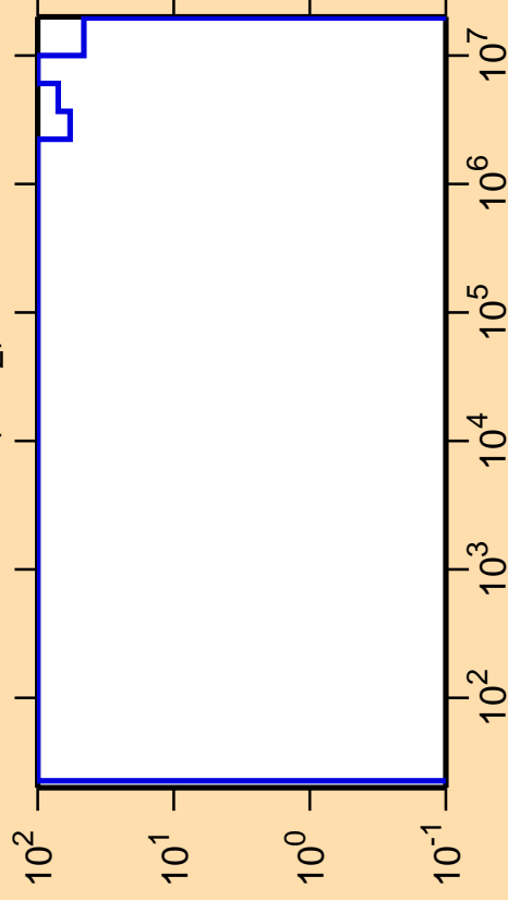
\Delta\sigma/\sigma vs. E for ^{198}\text{Bi}(n,n_2)
