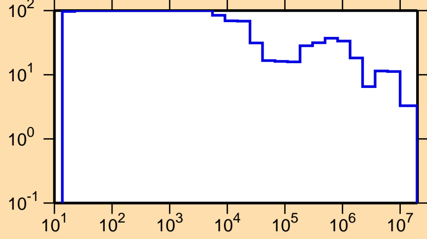
\Delta\sigma/\sigma vs. E for ^{198}\text{Bi}(n,\text{tot.})
