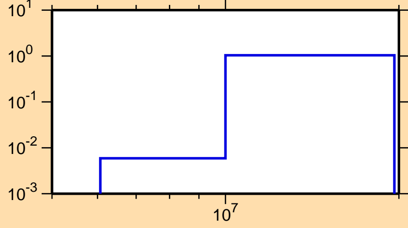
\sigma vs. E for ^{198}\text{Bi}(n,2n)
