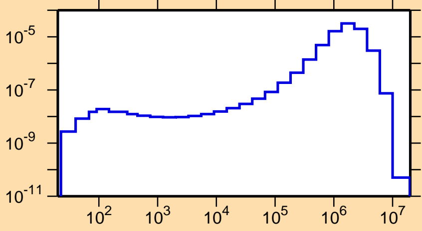
\sigma vs. E for ^{198}\text{Bi}(n,n_2)
