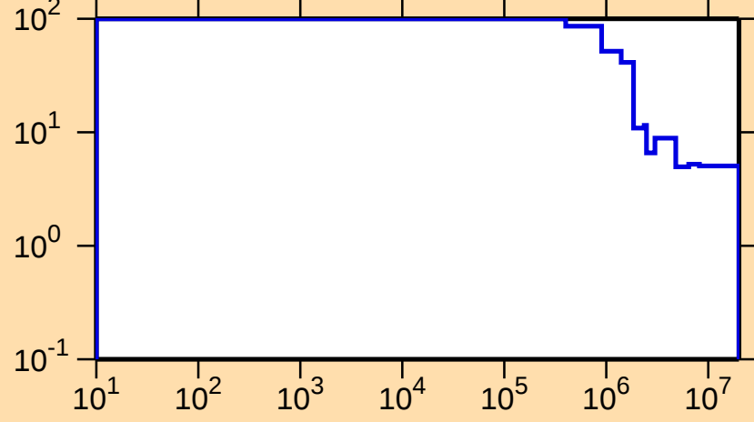
\Delta\sigma/\sigma vs. E for ^{198}\text{Bi}(n,\text{nonel.})
