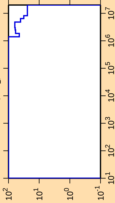
\Delta\sigma/\sigma vs. E for ^{198}\text{Bi}(n,n_1)
