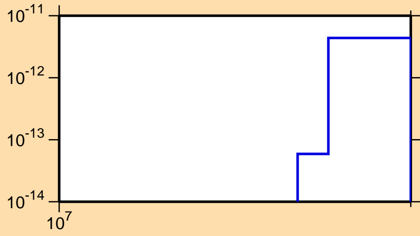
\sigma vs. E for ^{200}\text{Bi} (mt 34)
