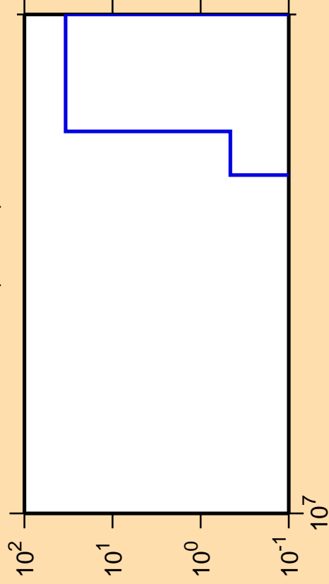
\Delta\sigma/\sigma vs. E for ^{200}\text{Bi} (mt 34)
