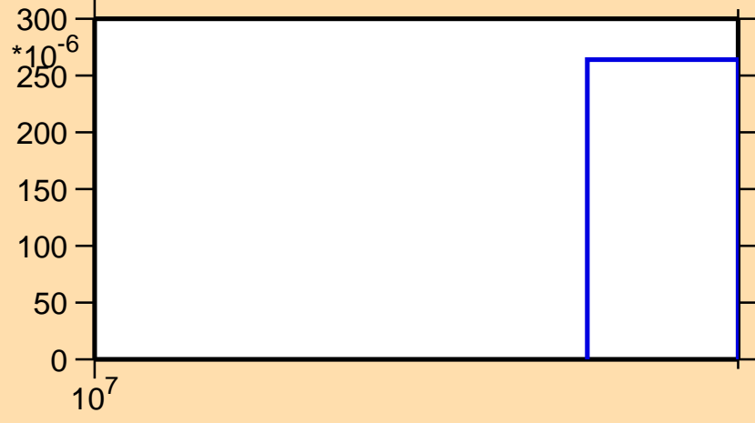
\sigma vs. E for ^{200}\text{Bi}(n,3n)
