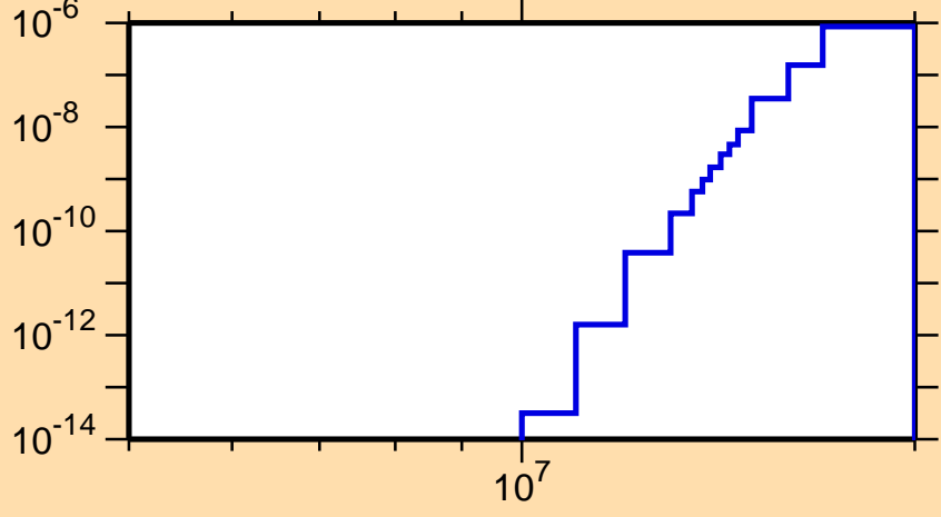
\sigma vs. E for ^{200}\text{Bi}(n,2n\alpha)
