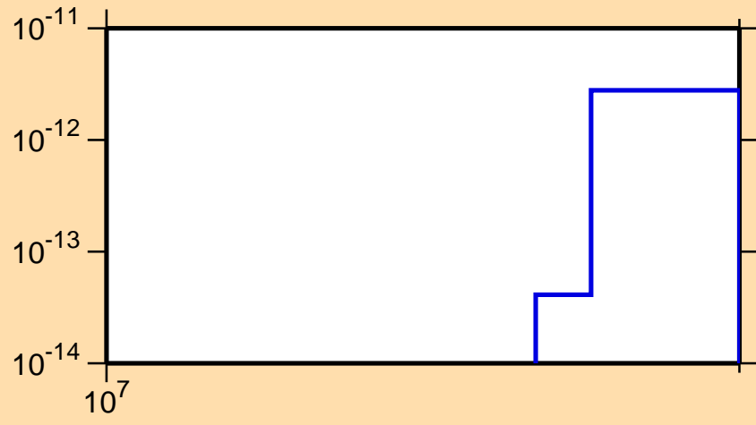
\sigma vs. E for ^{200}\text{Bi}(n,\text{pt})
