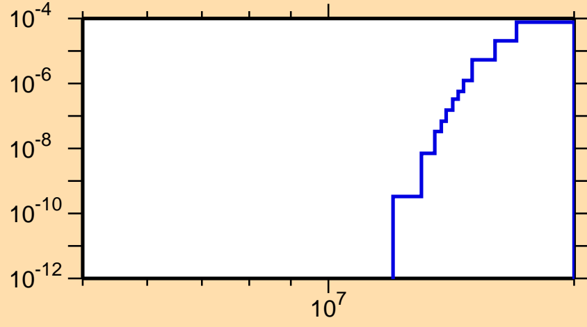
\sigma vs. E for ^{200}\text{Bi}(n,2np)
