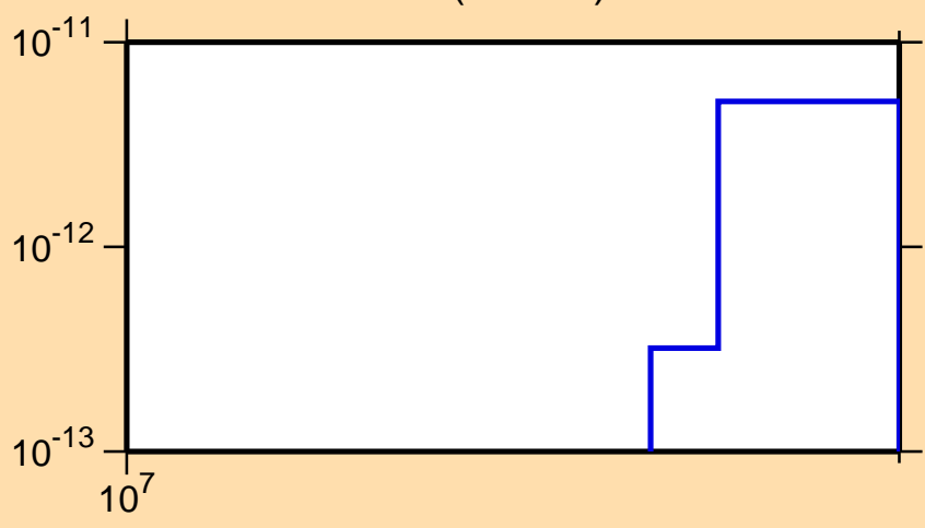
\sigma vs. E for ^{200}\text{Bi}(\text{mt117})
