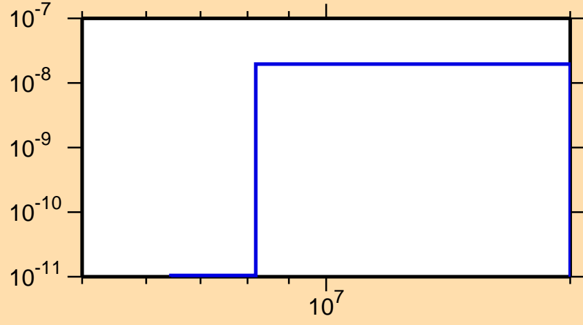
\sigma vs. E for ^{200}\text{Bi}(n,p\alpha)
