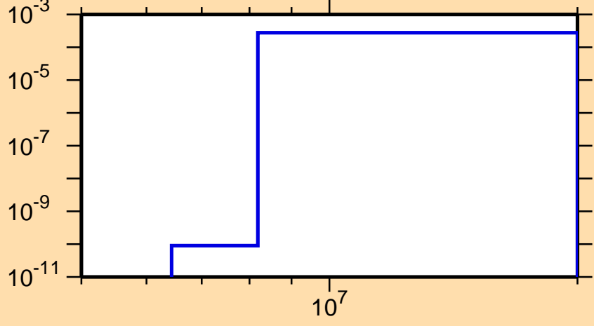
\sigma vs. E for ^{200}\text{Bi}(n,t)
