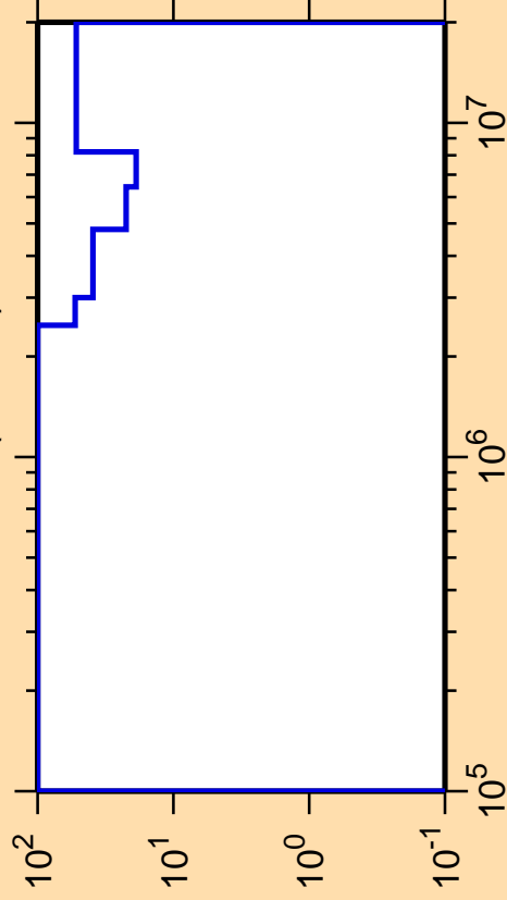
\Delta\sigma/\sigma vs. E for ^{200}\text{Bi}(n,\text{inel.})
