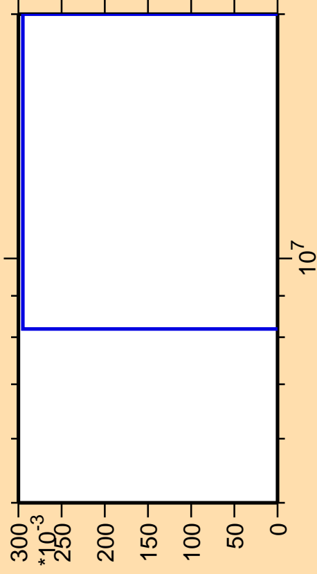
\Delta\sigma/\sigma vs. E for ^{200}\text{Bi}(\text{mt } 34)
