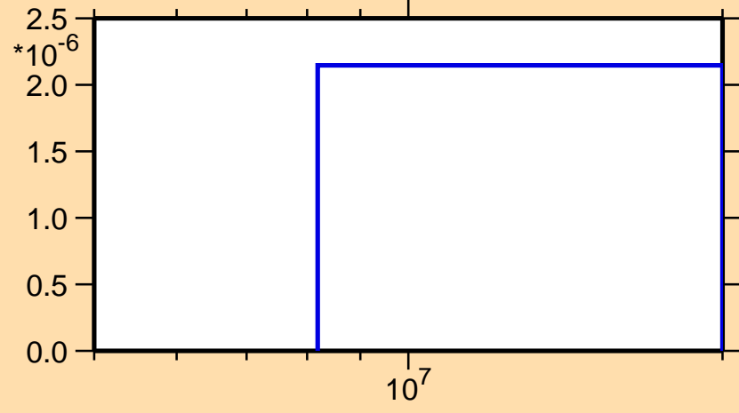
\sigma vs. E for ^{200}\text{Bi}(n,3n)
