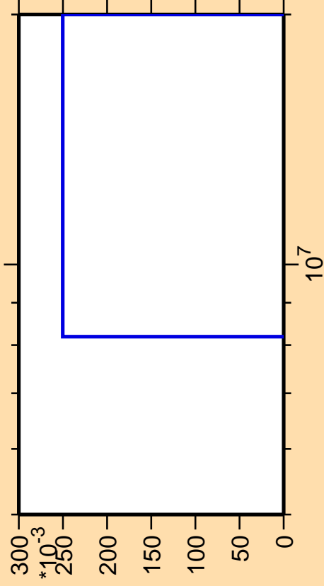
\Delta\sigma/\sigma vs. E for ^{200}\text{Bi}(\text{mt117})
