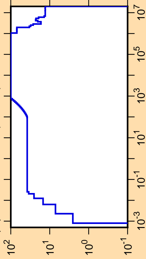
\Delta\mu/\mu vs. E for ^{201}\text{Bi}(\text{mt251})
