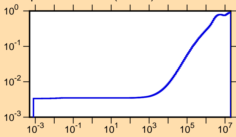
\mu vs. E for ^{201}\text{Bi}(\text{mt251})
