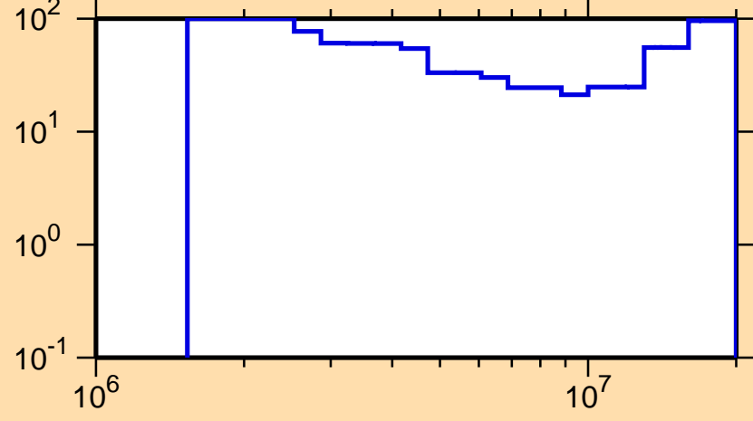
\Delta\sigma/\sigma vs. E for ^{201}\text{Bi}(n,n\text{cont.})
