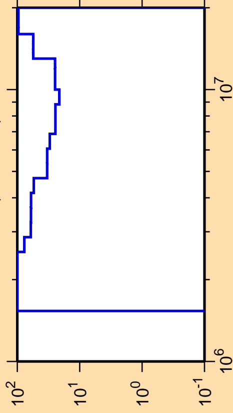
\Delta\sigma/\sigma vs. E for ^{201}\text{Bi}(n,n\text{cont.})
