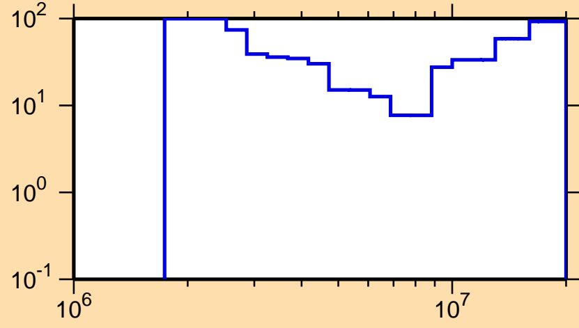
\Delta\sigma/\sigma vs. E for ^{203}\text{Bi}(n,n\text{cont.})
