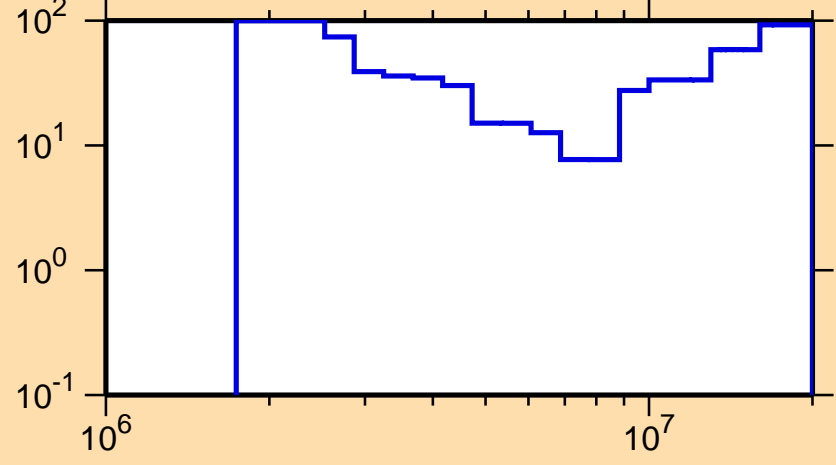
\Delta\sigma/\sigma vs. E for ^{203}\text{Bi}(n,ncont.)
