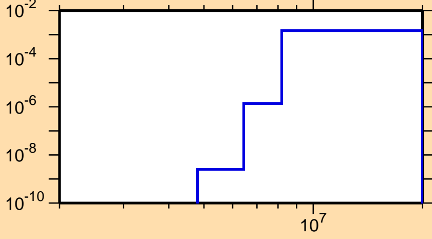
\sigma vs. E for ^{203}\text{Bi}(n,np)
