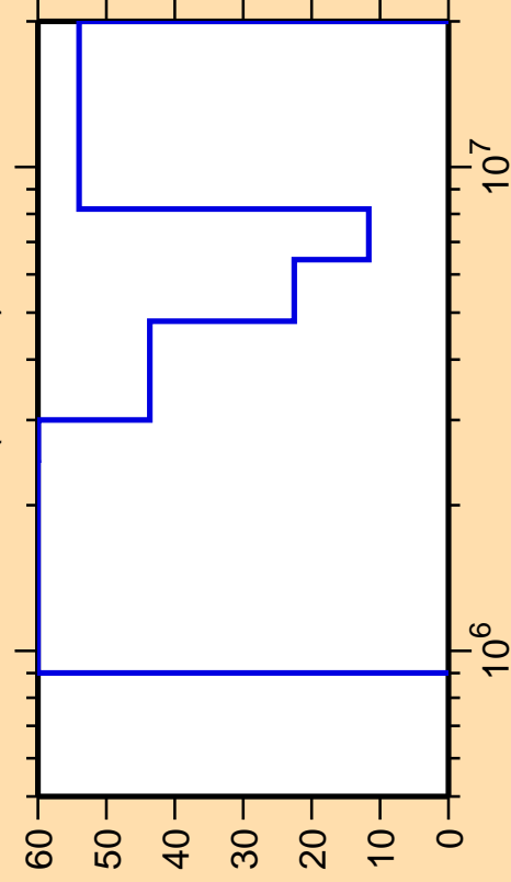
\Delta\sigma/\sigma vs. E for ^{203}\text{Bi}(n,\text{inel.})
