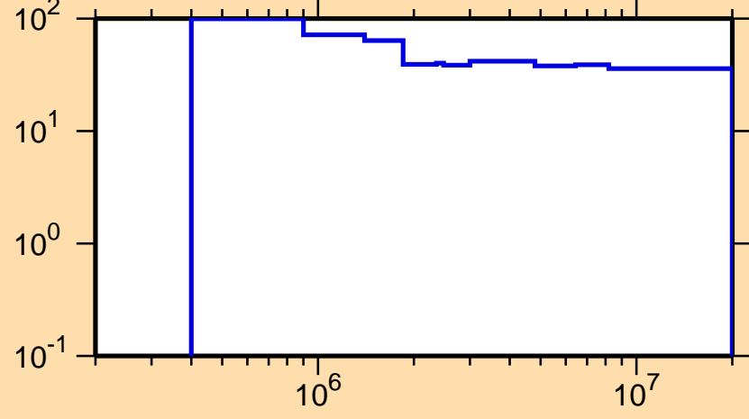
\Delta\sigma/\sigma vs. E for ^{203}\text{Bi}(n,n_1)
