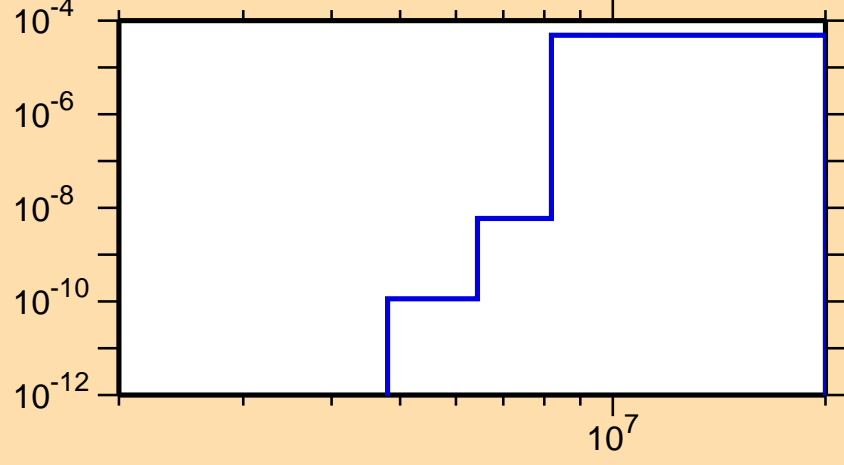
\sigma vs. E for ^{203}\text{Bi}(n,\alpha)
