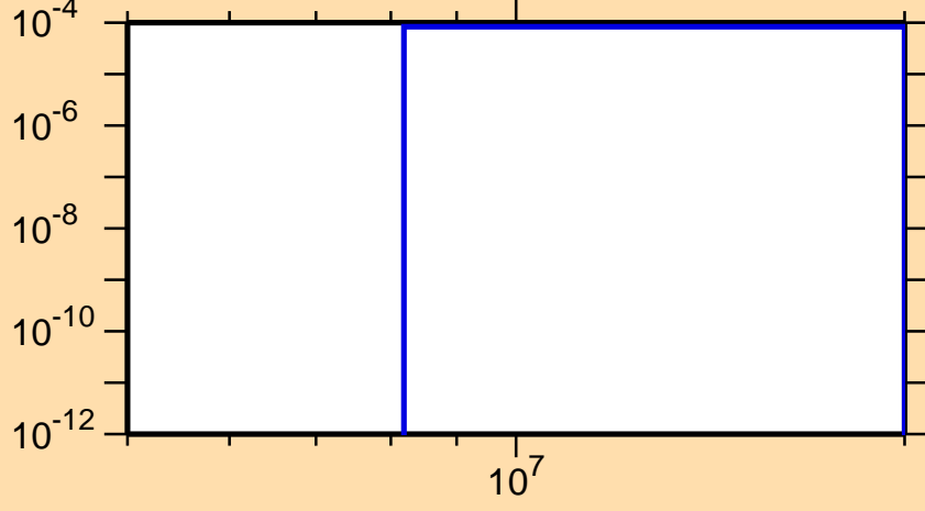
\sigma vs. E for ^{203}\text{Bi}(n,t)
