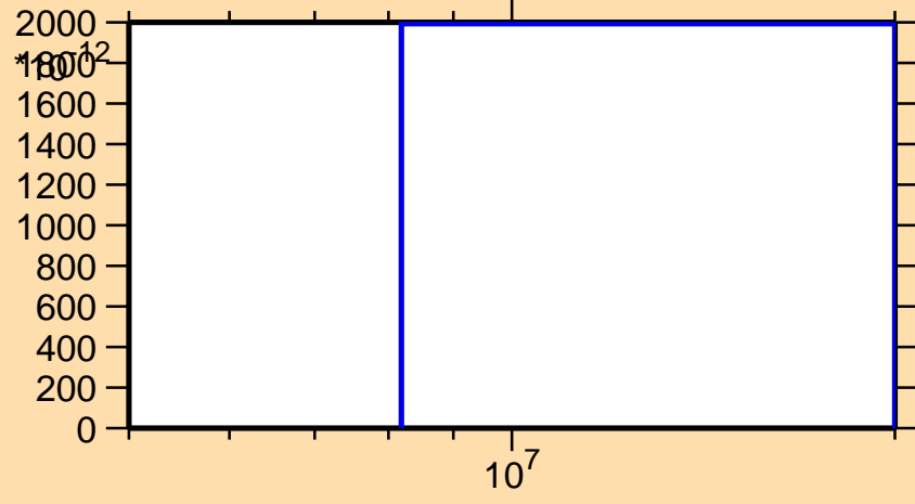
\sigma vs. E for ^{203}\text{Bi}(n,\text{He}3)
