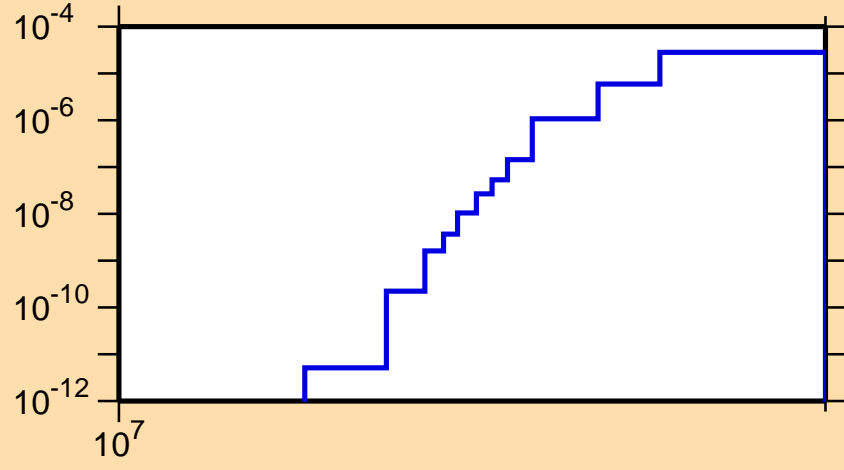
\sigma vs. E for ^{204}\text{Bi}(n,2np)
