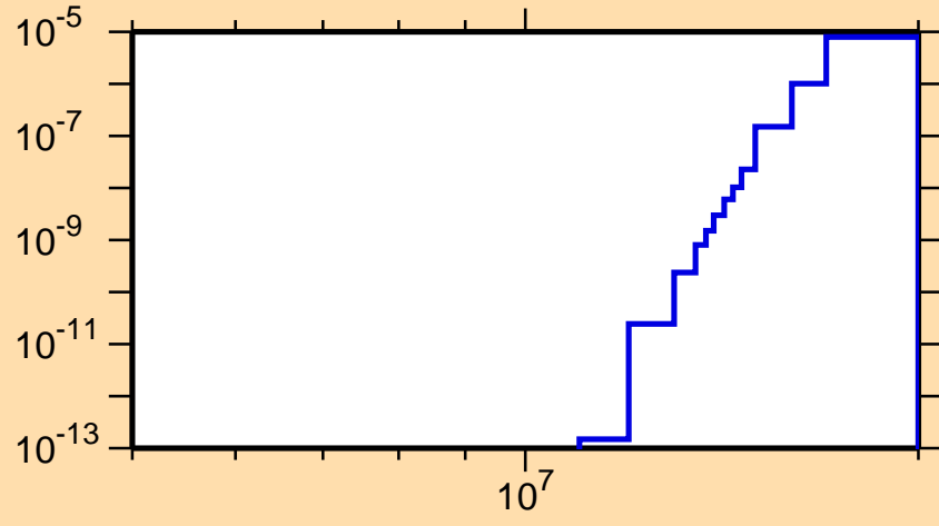
\sigma vs. E for ^{204}\text{Bi}(n,\text{nd})
