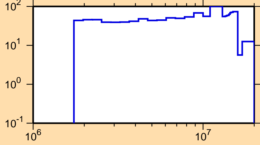
\Delta\sigma/\sigma vs. E for ^{204}\text{Bi}(n,n_1)
