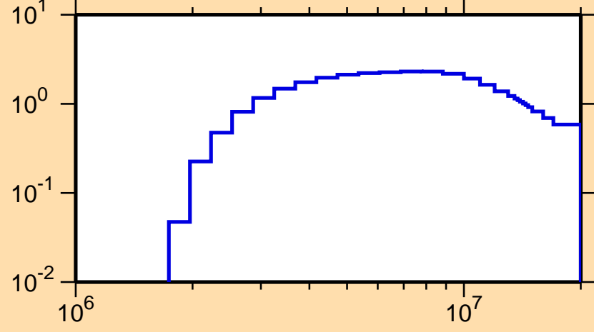
\sigma vs. E for ^{204}\text{Bi}(n,n\text{cont.})
