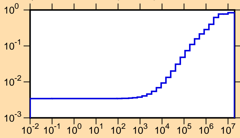
\mu vs. E for ^{204}\text{Bi}(\text{mt251})
