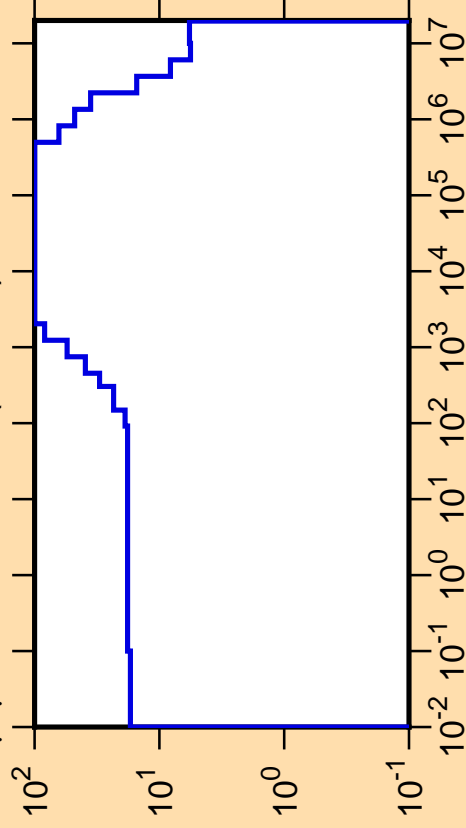
\Delta\mu/\mu vs. E for ^{204}\text{Bi}(\text{mt251})
