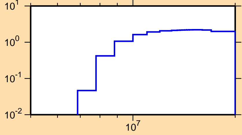
\sigma vs. E for ^{206}\text{Bi}(n,2n)
