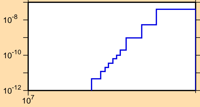
\sigma vs. E for ^{206}\text{Bi}(n,\text{He3})
