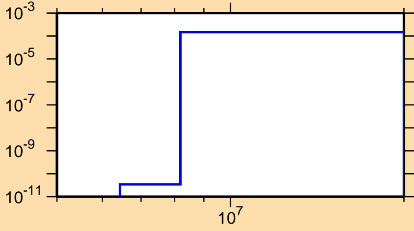
\sigma vs. E for ^{206}\text{Bi}(n,t)
