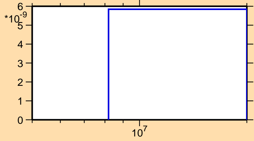
\sigma vs. E for ^{206}\text{Bi}(n,2n\alpha)
