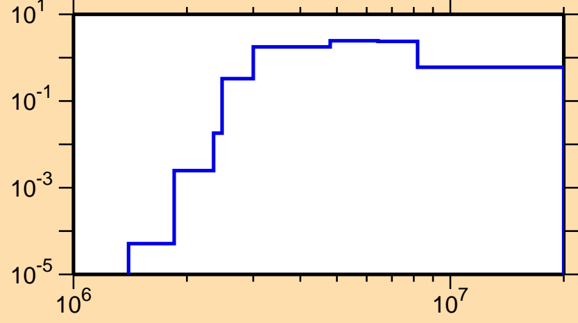
\sigma vs. E for ^{206}\text{Bi}(n,n\text{cont.})
