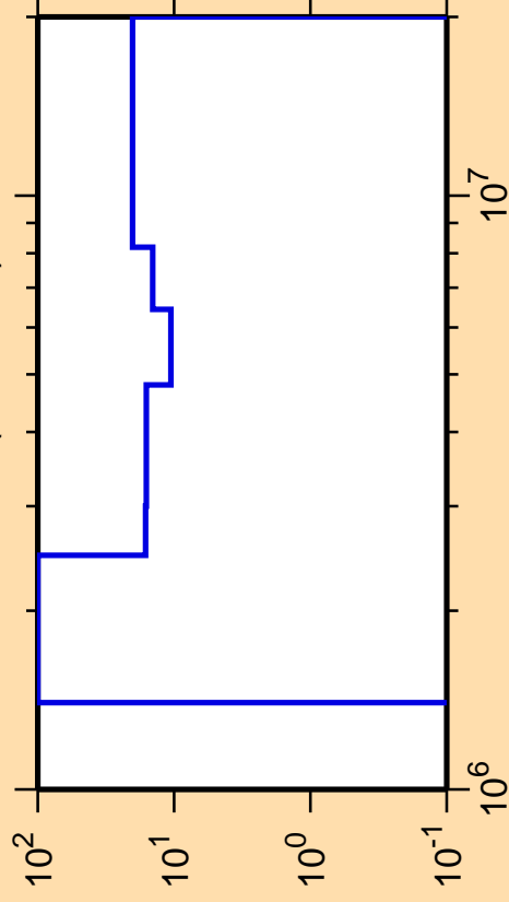
\Delta\sigma/\sigma vs. E for ^{206}\text{Bi}(n,\text{ncont.})
