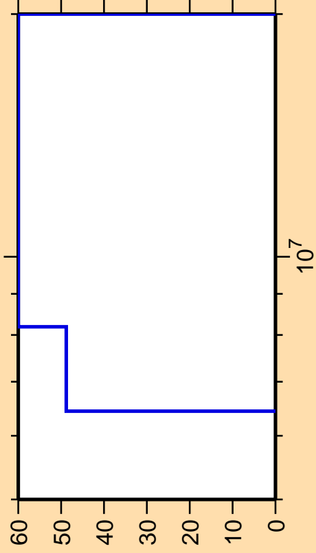
\Delta\sigma/\sigma vs. E for ^{206}\text{Bi}(n,\gamma)
