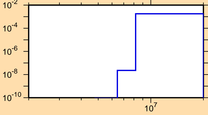
\sigma vs. E for ^{206}\text{Bi}(n,d)
