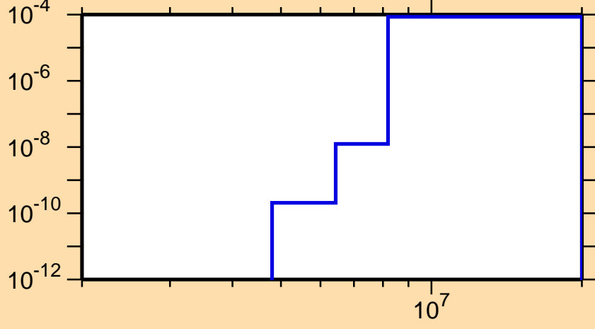
\sigma vs. E for ^{206}\text{Bi}(n,\alpha)
