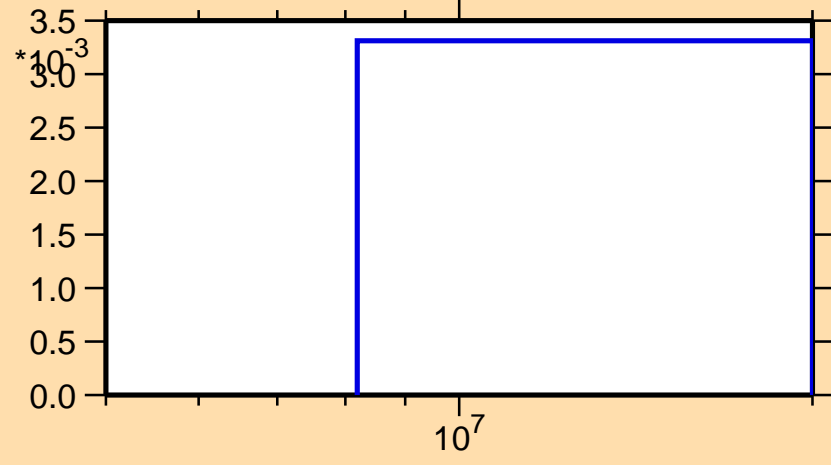
\sigma vs. E for ^{206}\text{Bi}(n,3n)
