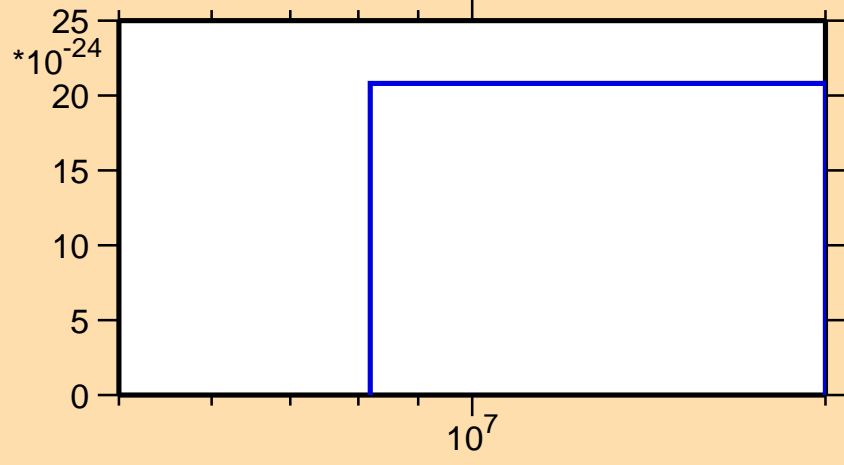
\sigma vs. E for ^{206}\text{Bi} (mt 42)
