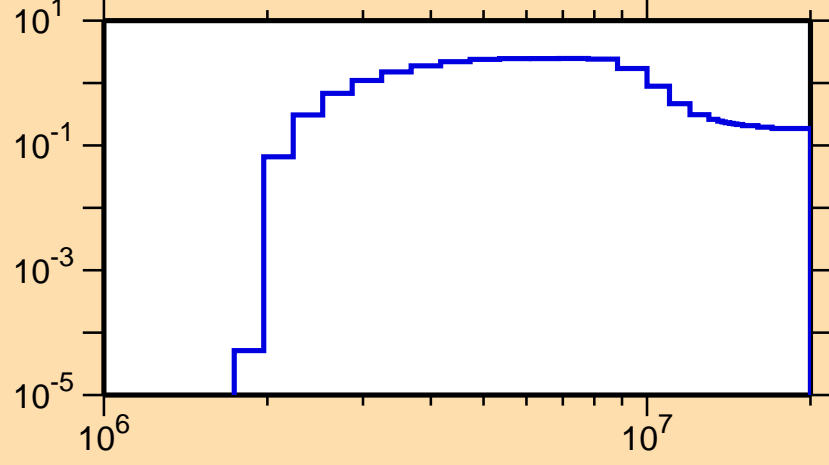
\sigma vs. E for ^{207}\text{Bi}(n,n\text{cont.})
