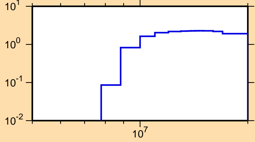
\sigma vs. E for ^{207}\text{Bi}(n,2n)
