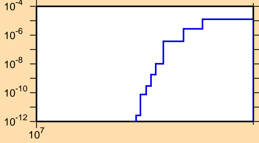
\sigma vs. E for ^{207}\text{Bi}(n,2np)
