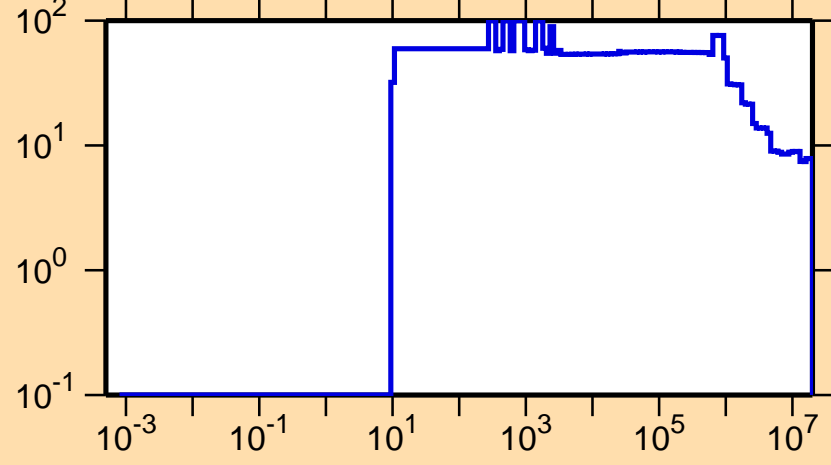
\Delta\sigma/\sigma vs. E for ^{207}\text{Bi}(n,\text{nonel.})
