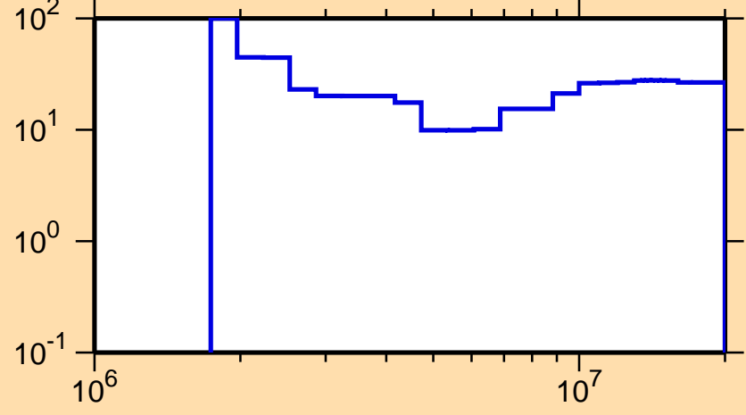
\Delta\sigma/\sigma vs. E for ^{207}\text{Bi}(n,n\text{cont.})
