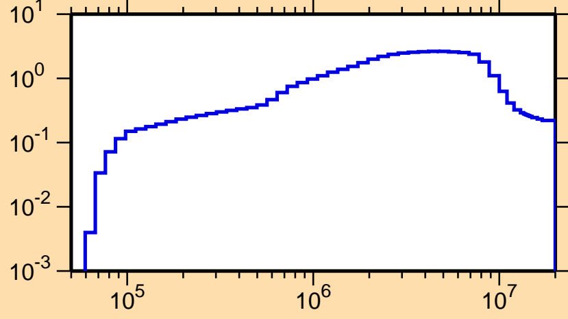
\sigma vs. E for ^{208}\text{Bi}(n,\text{inel.})
