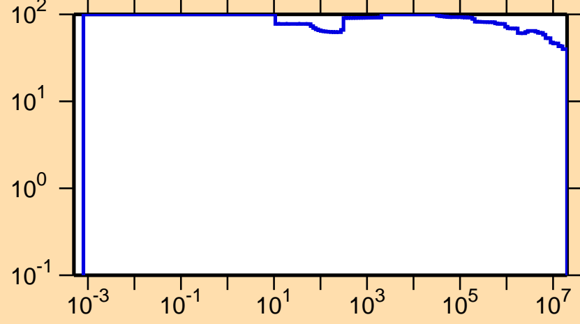
\Delta\sigma/\sigma vs. E for ^{208}\text{Bi}(n,p)
