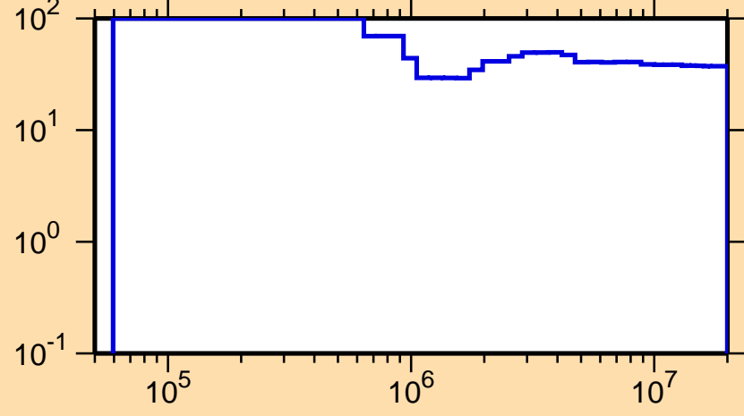
\Delta\sigma/\sigma vs. E for ^{208}\text{Bi}(n,n_1)
