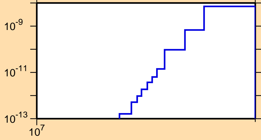
\sigma vs. E for ^{208}\text{Bi}(n,\text{He3})
