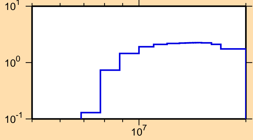
\sigma vs. E for ^{208}\text{Bi}(n,2n)
