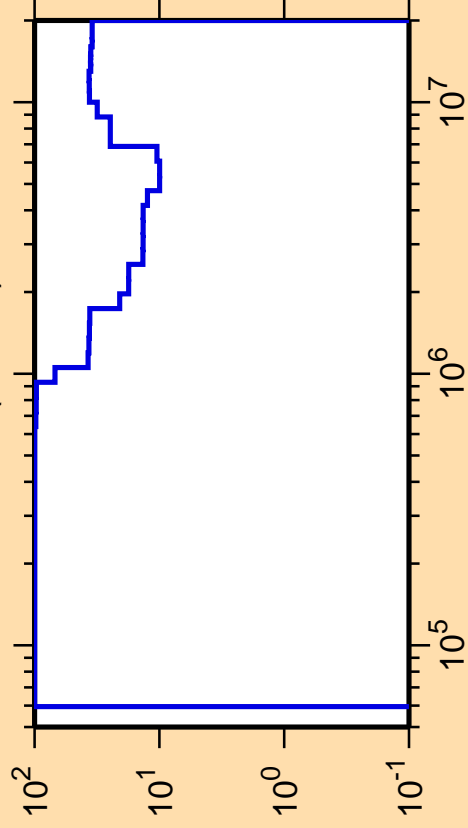
\Delta\sigma/\sigma vs. E for ^{208}\text{Bi}(n,\text{inel.})
