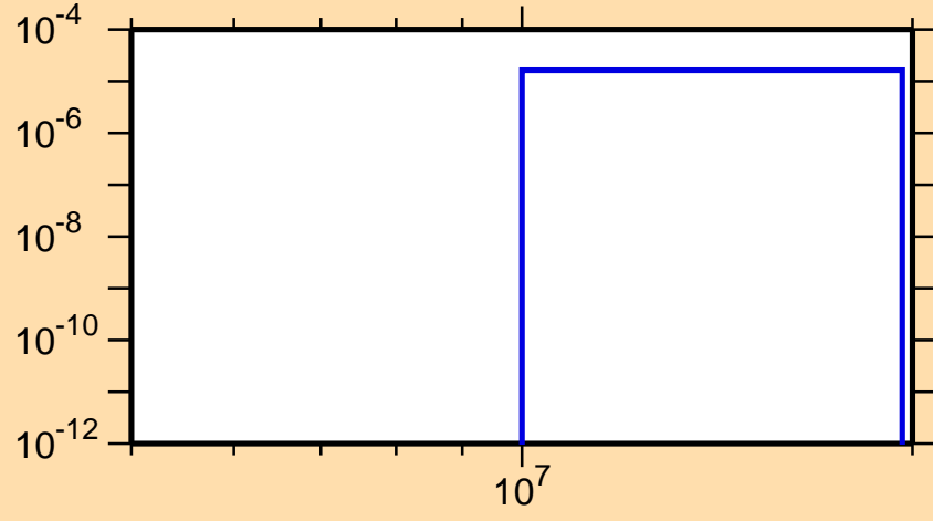
\sigma vs. E for ^{210}\text{Bi}(n,2np)
