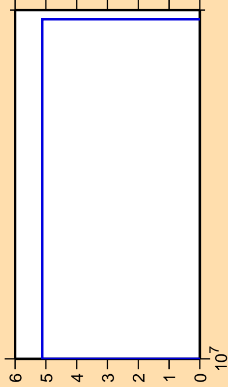
\Delta\sigma/\sigma vs. E for ^{210}\text{Bi}(n,p\alpha)
