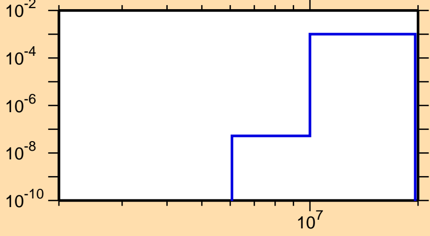
\sigma vs. E for ^{210}\text{Bi}(n,d)
