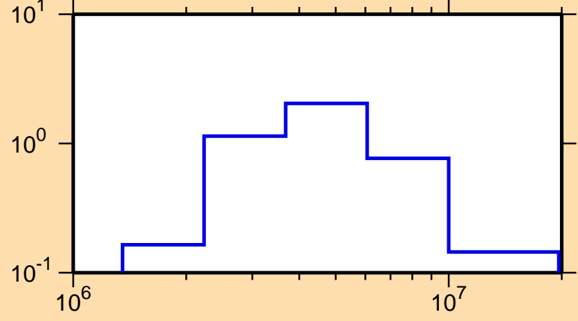
\sigma vs. E for ^{210}\text{Bi}(n,n\text{cont.})
