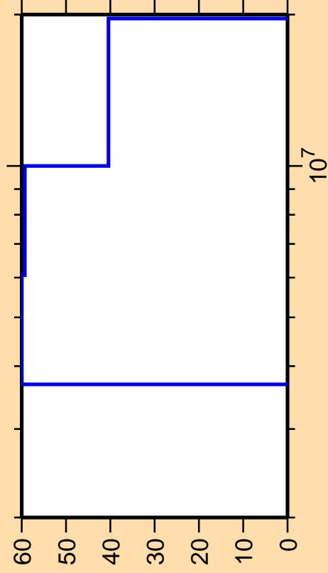
\Delta\sigma/\sigma vs. E for ^{210}\text{Bi}(n,p)
