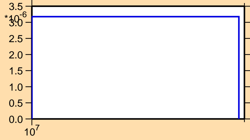
\sigma vs. E for ^{210}\text{Bi}(n,\text{nt})
