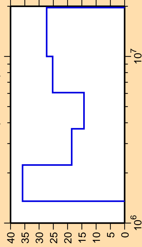
\Delta\sigma/\sigma vs. E for ^{210}\text{Bi}(n,\text{ncont.})
