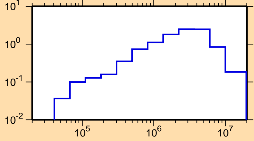
\sigma vs. E for ^{210}\text{Bi}(n,\text{inel.})
