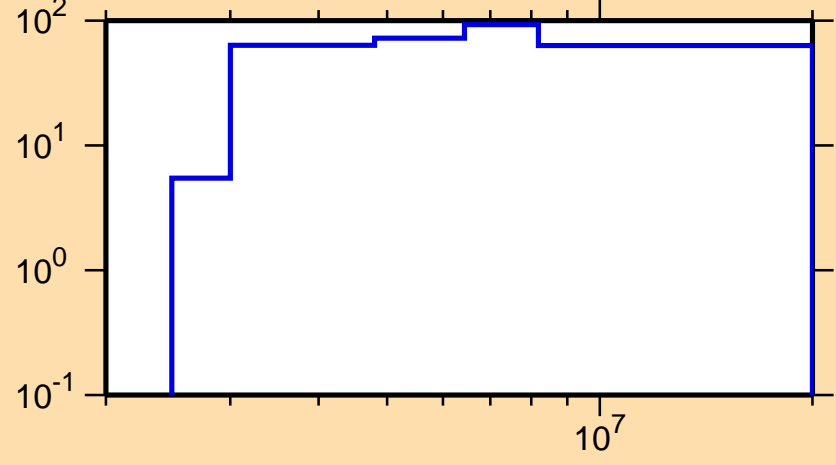
\Delta\sigma/\sigma vs. E for ^{210}\text{Bi}(n,p)
