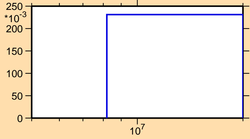
\sigma vs. E for ^{210}\text{Bi}(n,3n)
