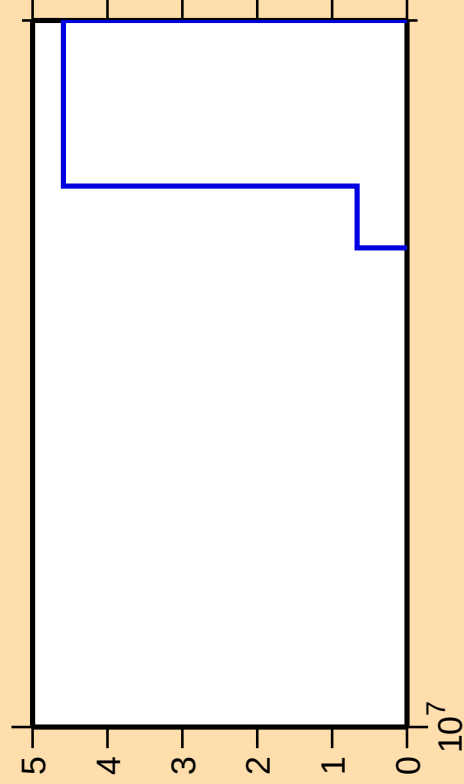
\Delta\sigma/\sigma vs. E for ^{212}\text{Bi}(n,p\alpha)
