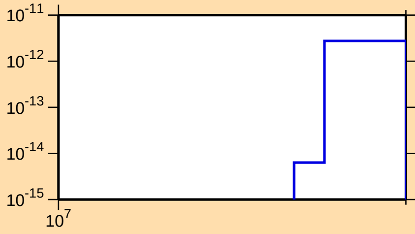
\sigma vs. E for ^{212}\text{Bi}(\text{mt } 45)
