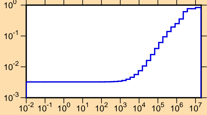
\mu vs. E for ^{212}\text{Bi}(\text{mt251})
