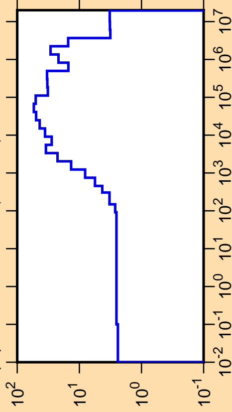
\Delta\mu/\mu vs. E for ^{212}\text{Bi}(\text{mt251})
