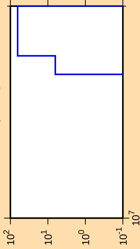
\Delta\sigma/\sigma vs. E for ^{215}\text{Bi}(\text{mt } 42)
