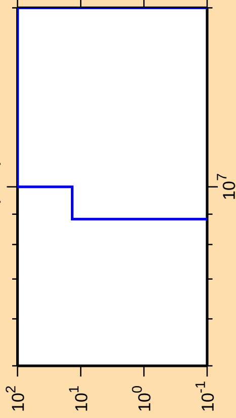
\Delta\sigma/\sigma vs. E for ^{215}\text{Bi}(n,\text{nt})
