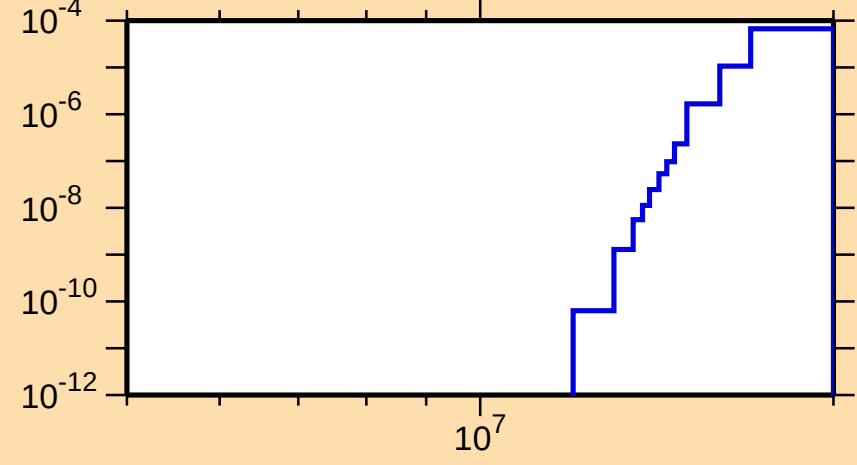
\sigma vs. E for ^{215}\text{Bi}(n,2np)
