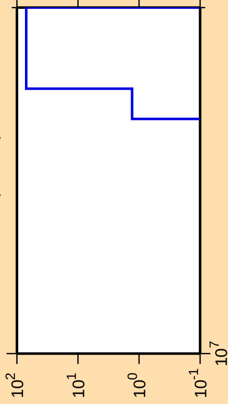
\Delta\sigma/\sigma vs. E for ^{215}\text{Bi}(n,\text{He3})
