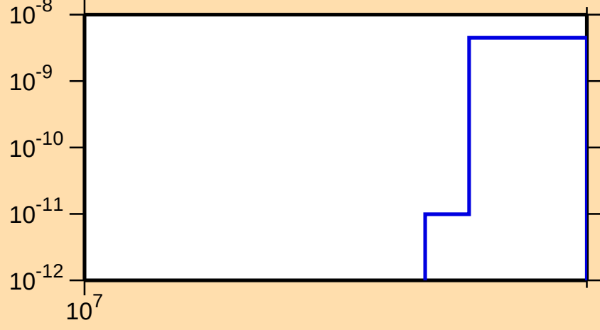
\sigma vs. E for ^{215}\text{Bi}(\text{mt } 42)
