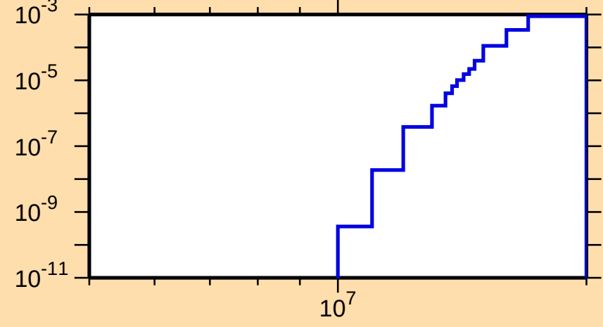
\sigma vs. E for ^{215}\text{Bi}(n,\text{nt})
