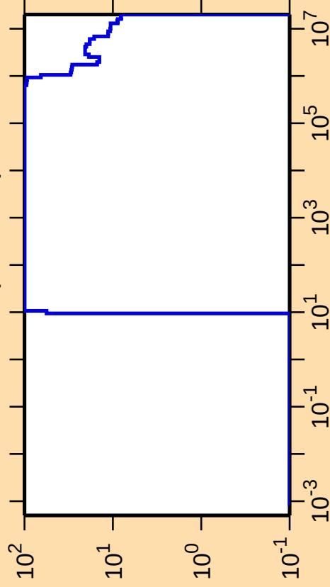
\Delta\sigma/\sigma vs. E for ^{215}\text{Bi}(n,\text{nonel.})
