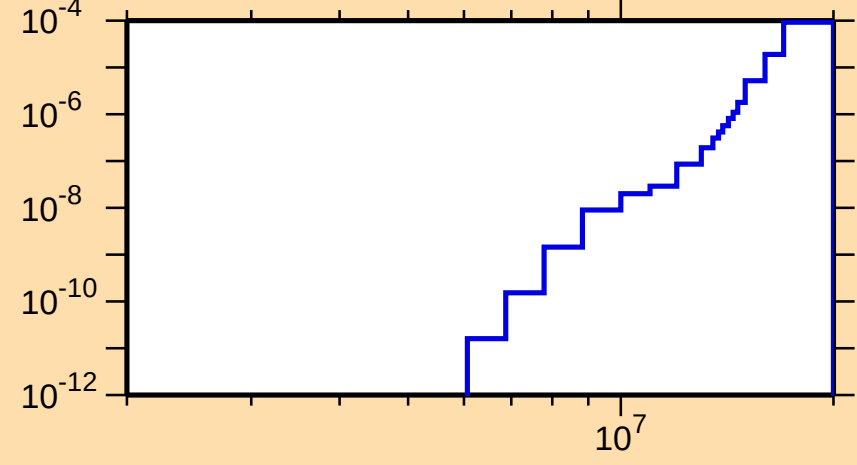
\sigma vs. E for ^{215}\text{Bi}(n,2n\alpha)
