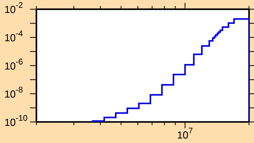
\sigma vs. E for ^{216}\text{Bi}(n,n\alpha)
