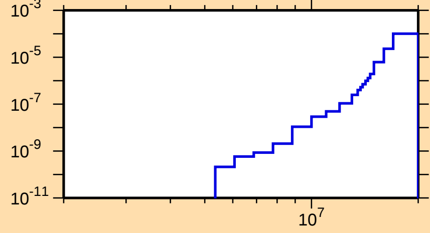
\sigma vs. E for ^{216}\text{Bi}(n,2n\alpha)
