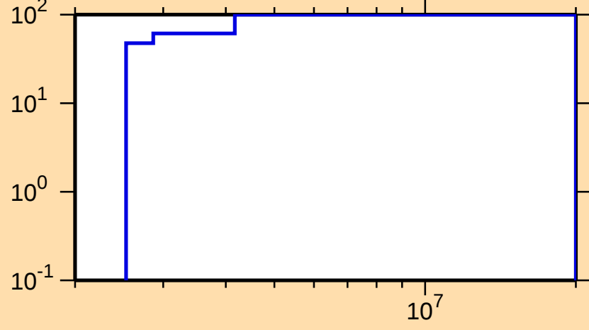
\Delta\sigma/\sigma vs. E for ^{216}\text{Bi}(n,n\text{cont.})
