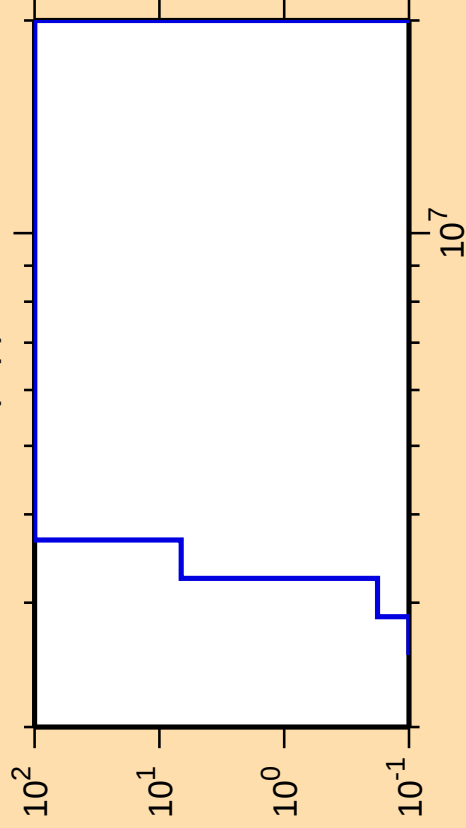
\Delta\sigma/\sigma vs. E for ^{216}\text{Bi}(n,p)
