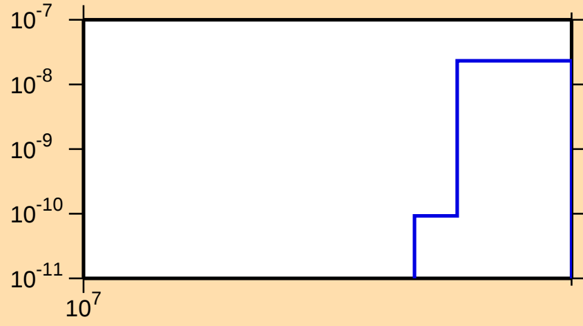
\sigma vs. E for ^{216}\text{Bi}(\text{mt 11})
