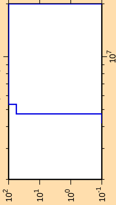
\Delta\sigma/\sigma vs. E for ^{216}\text{Bi}(n,2n\alpha)
