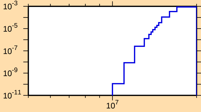
\sigma vs. E for ^{216}\text{Bi}(n,\text{nt})
