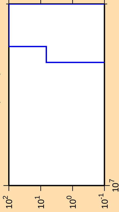
\Delta\sigma/\sigma vs. E for ^{216}\text{Bi}(\text{mt } 42)
