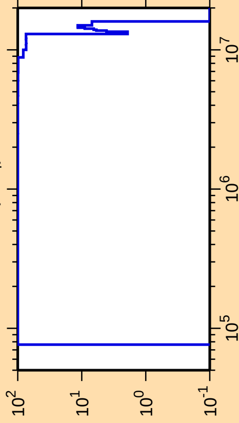
\Delta\sigma/\sigma vs. E for ^{216}\text{Bi}(n,n_4)
