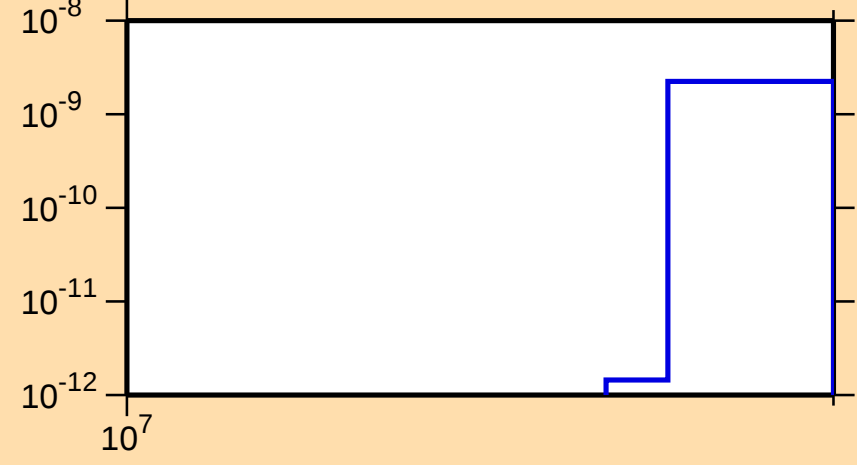
\sigma vs. E for ^{216}\text{Bi}(\text{mt } 42)
