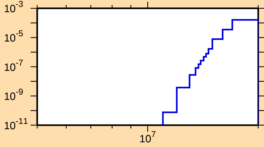
\sigma vs. E for ^{216}\text{Bi}(n,\text{nd})
