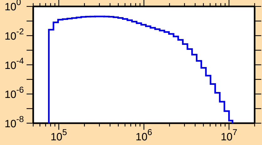
\sigma vs. E for ^{216}\text{Bi}(n,n_4)
