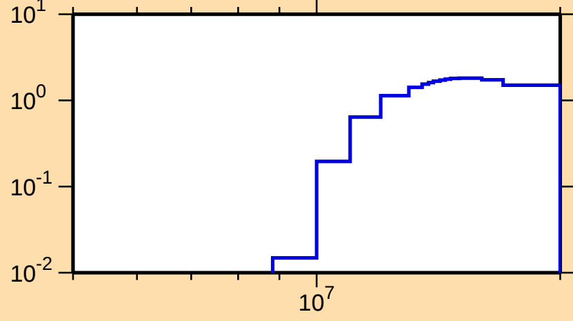
\sigma vs. E for ^{216}\text{Bi}(n,3n)
