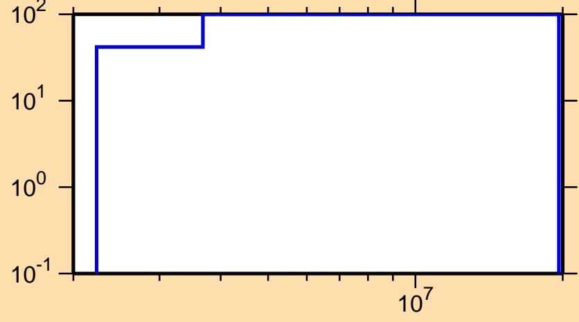
\Delta\sigma/\sigma vs. E for ^{216}\text{Bi}(n,ncont.)
