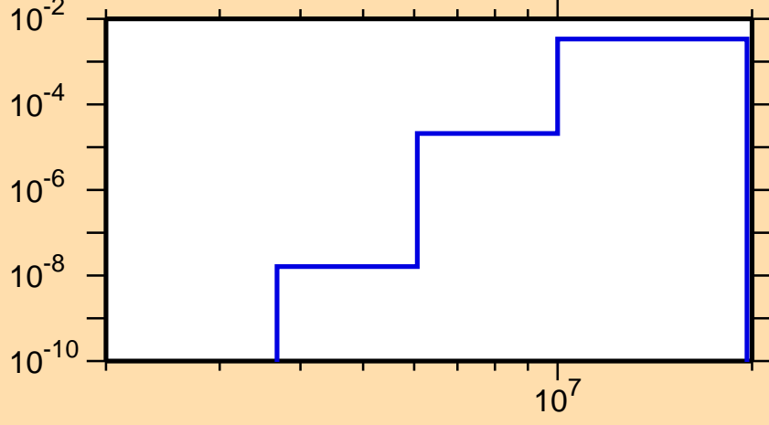
\sigma vs. E for ^{216}\text{Bi}(n,p)
