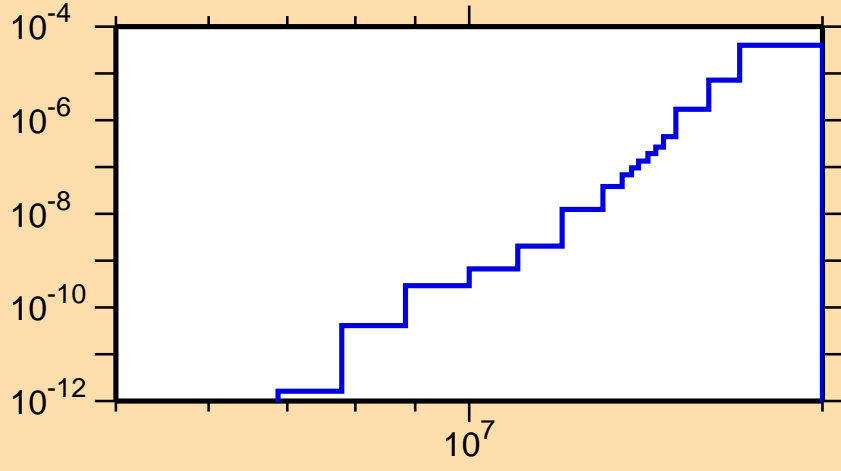
\sigma vs. E for ^{218}\text{Bi}(n,2n\alpha)
