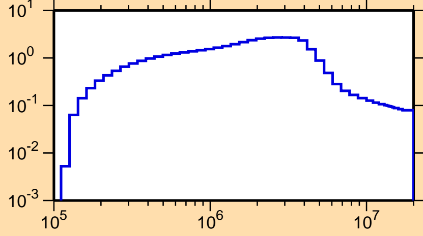
\sigma vs. E for ^{218}\text{Bi}(n,\text{inel.})
