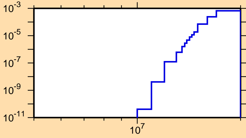
\sigma vs. E for ^{218}\text{Bi}(n,\text{nt})
