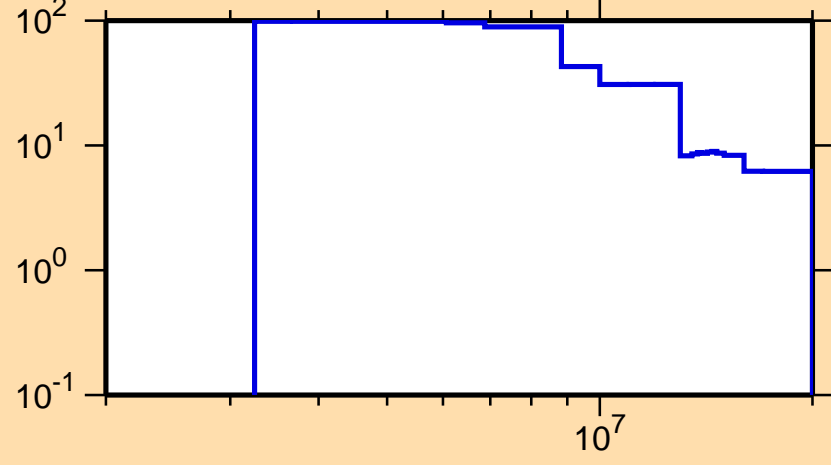
\Delta\sigma/\sigma vs. E for ^{218}\text{Bi}(n,2n)
