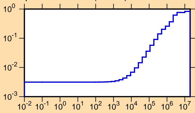
\mu vs. E for ^{218}\text{Bi}(\text{mt251})
