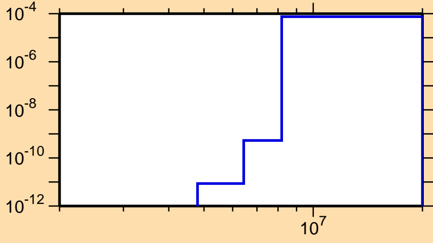
\sigma vs. E for ^{218}\text{Bi}(n,n\alpha)
