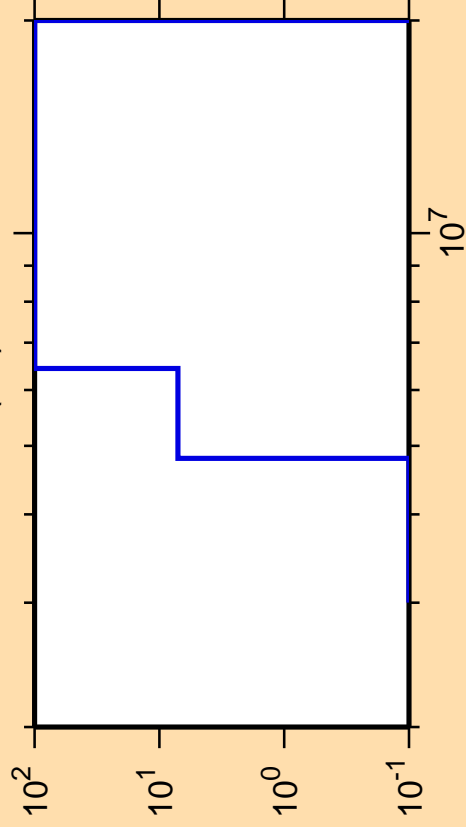
\Delta\sigma/\sigma vs. E for ^{218}\text{Bi}(n,t)
