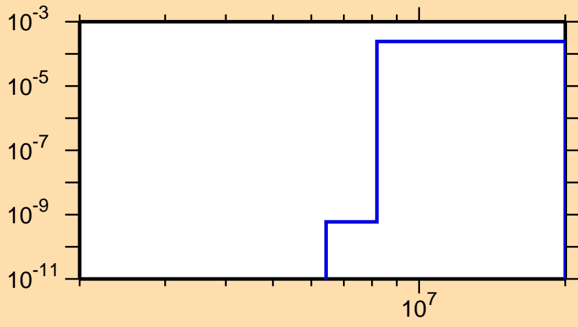
\sigma vs. E for ^{218}\text{Bi}(n,t)
