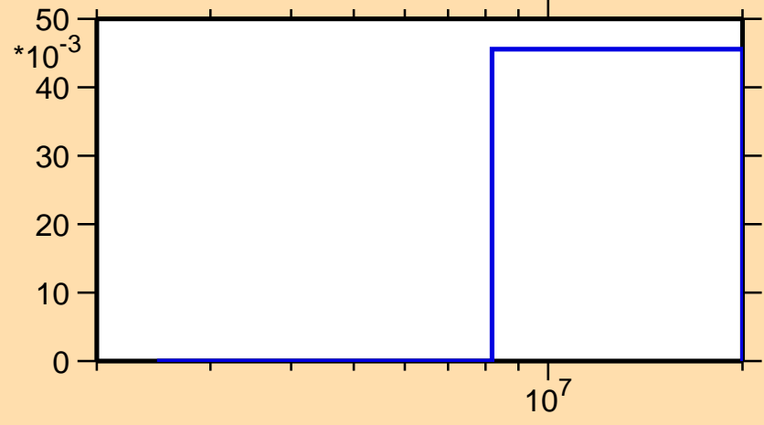
\Delta\sigma/\sigma vs. E for ^{218}\text{Bi}(n,f)
