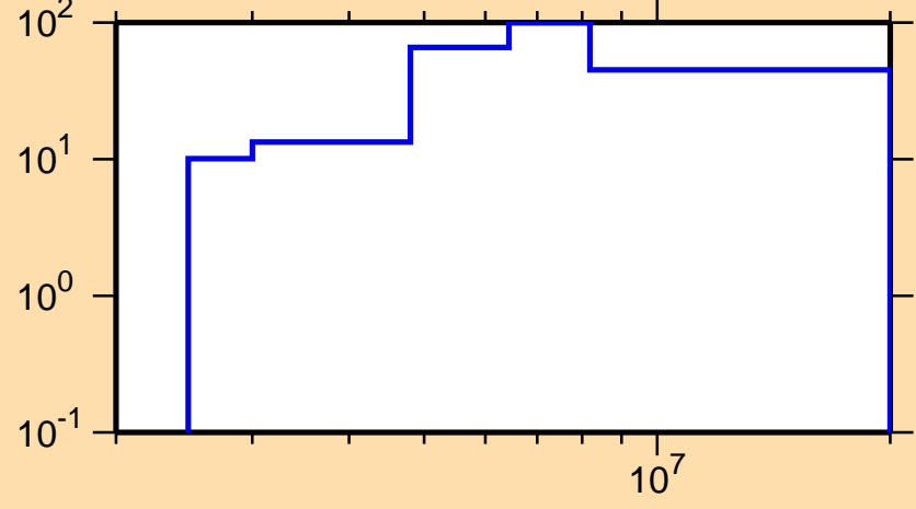
\Delta\sigma/\sigma vs. E for ^{218}\text{Bi}(n,\text{el.})
