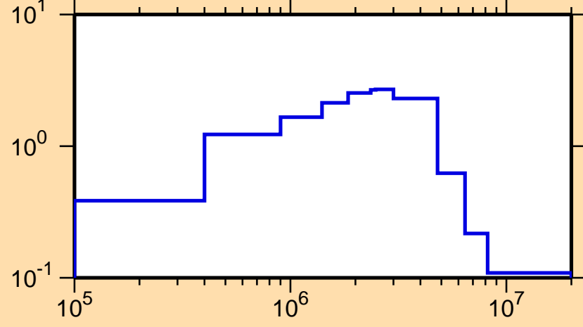
\sigma vs. E for ^{218}\text{Bi}(n,\text{inel.})
