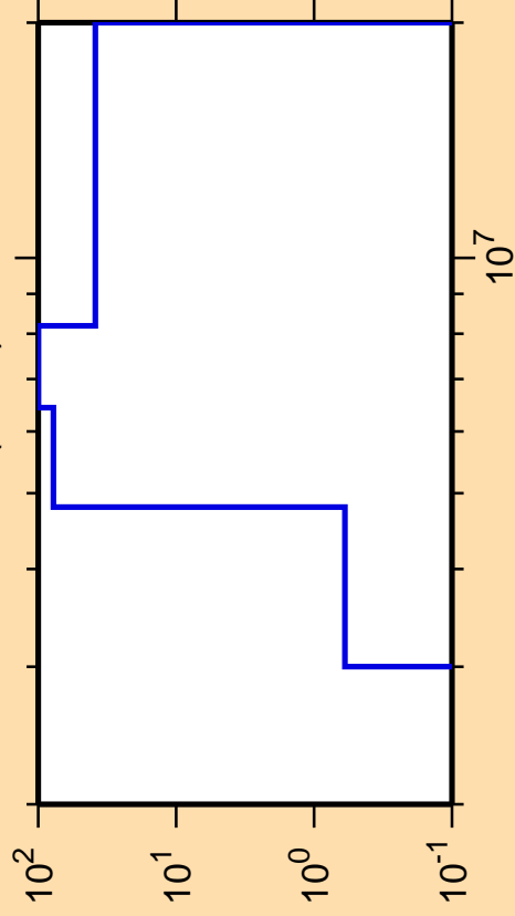
\Delta\sigma/\sigma vs. E for ^{218}\text{Bi}(n,n\alpha)
