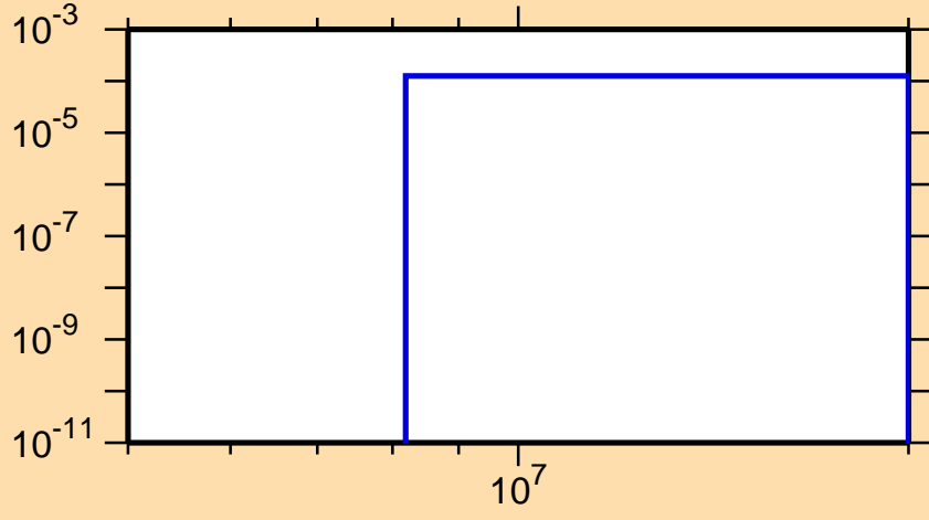
\sigma vs. E for ^{218}\text{Bi}(n,d)
