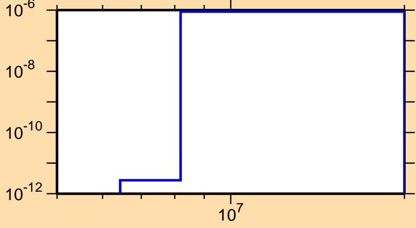
\sigma vs. E for ^{218}\text{Bi}(n,2n\alpha)
