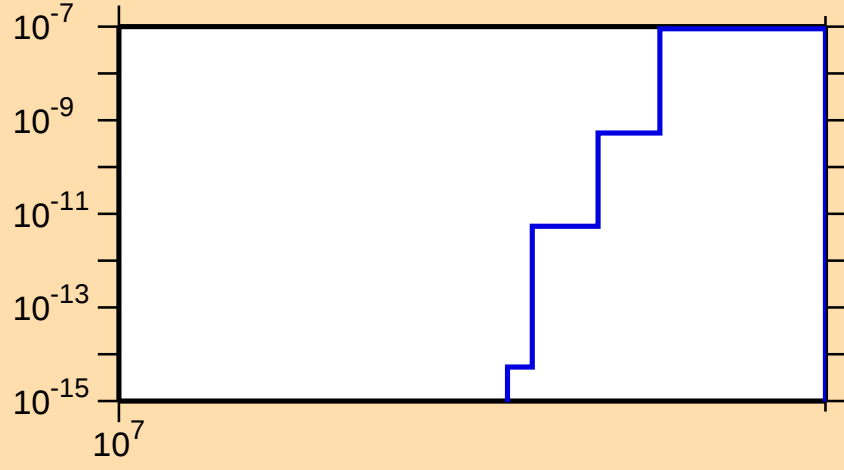
\sigma vs. E for ^{223}\text{Bi}(n,\text{nd})
