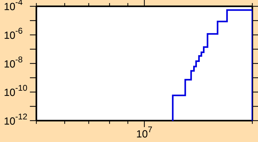
\sigma vs. E for ^{223}\text{Bi}(n,\text{nt})
