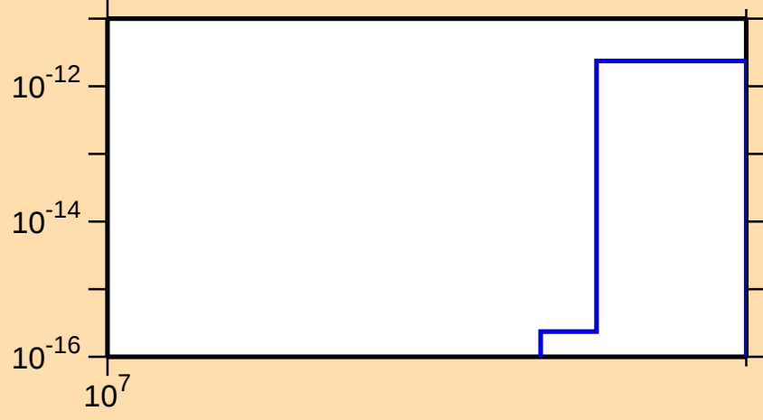
\sigma vs. E for ^{223}\text{Bi}(\text{mt } 42)
