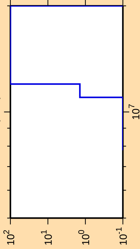
\Delta\sigma/\sigma vs. E for ^{223}\text{Bi}(n,\text{nt})
