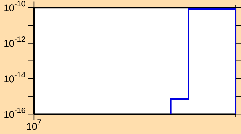
\sigma vs. E for ^{223}\text{Bi}(\text{mt 11})
