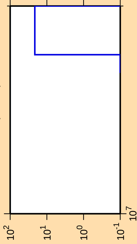
\Delta\sigma/\sigma vs. E for ^{223}\text{Bi}(\text{mt } 42)
