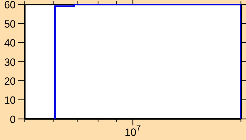
\Delta\sigma/\sigma vs. E for ^{223}\text{Bi}(n,\text{ncont.})
