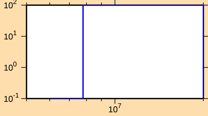
\Delta\sigma/\sigma vs. E for ^{223}\text{Bi}(n,p)
