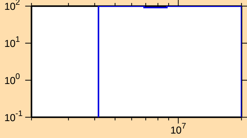
\Delta\sigma/\sigma vs. E for ^{223}\text{Bi}(n,2n)
