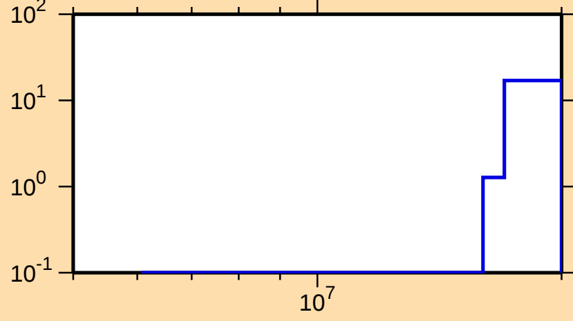
\Delta\sigma/\sigma vs. E for ^{223}\text{Bi}(n,f)
