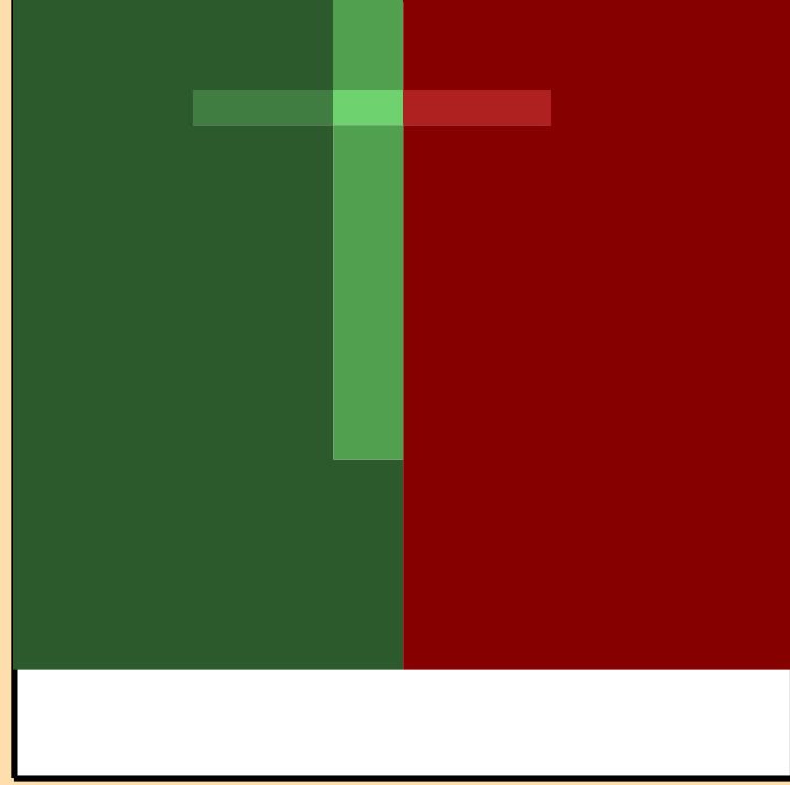
\Delta\sigma/\sigma vs. E for ^{223}\text{Bi}(n,n_1)
