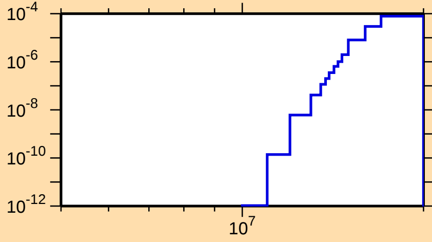
\sigma vs. E for ^{223}\text{Bi}(n,t)
