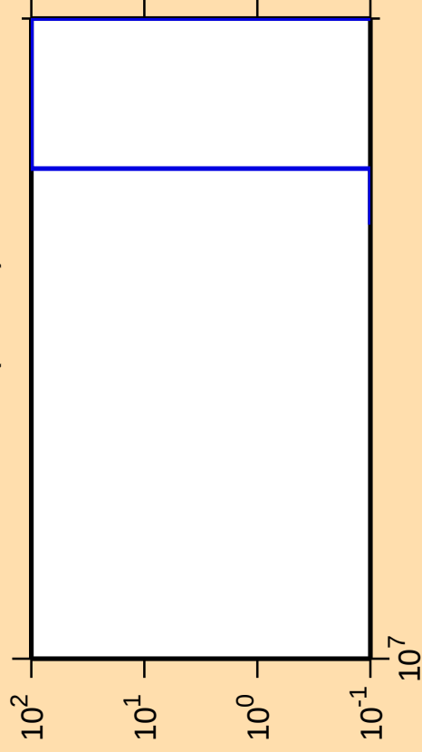
\Delta\sigma/\sigma vs. E for ^{223}\text{Bi}(\text{mt 11})
