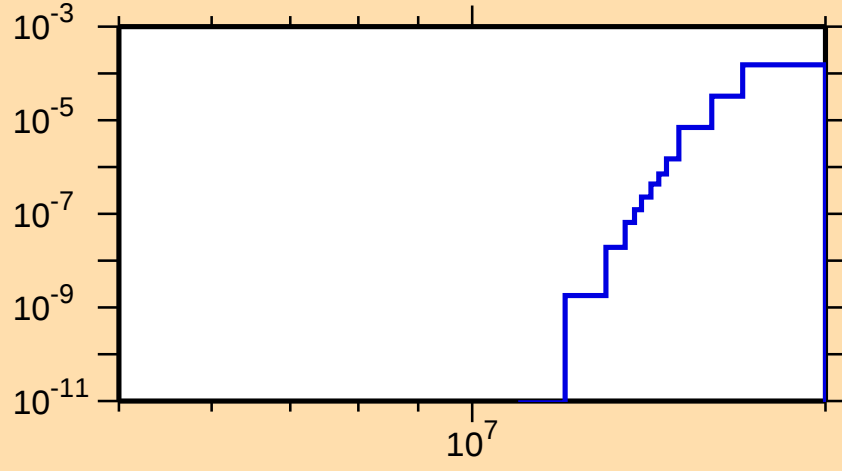
\sigma vs. E for ^{223}\text{Bi}(n,np)
