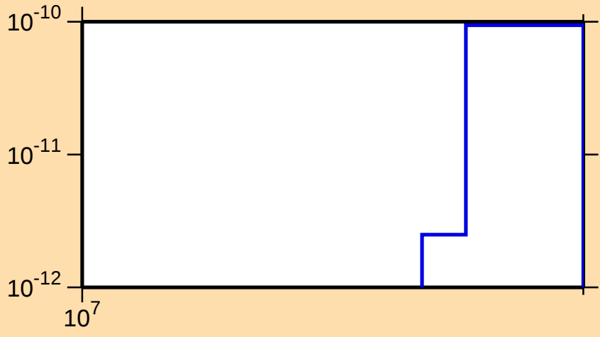
\sigma vs. E for ^{223}\text{Bi}(n,3n\alpha)
