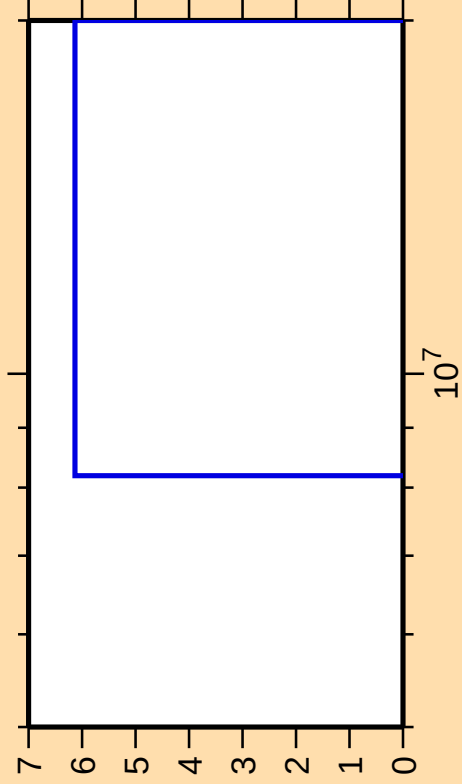
\Delta\sigma/\sigma vs. E for ^{223}\text{Bi}(\text{mt } 11)
