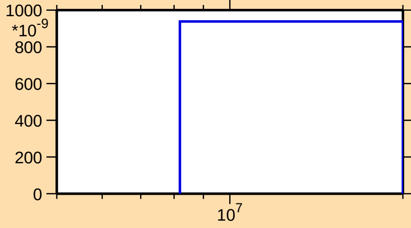
\sigma vs. E for ^{223}\text{Bi}(n,nt)
