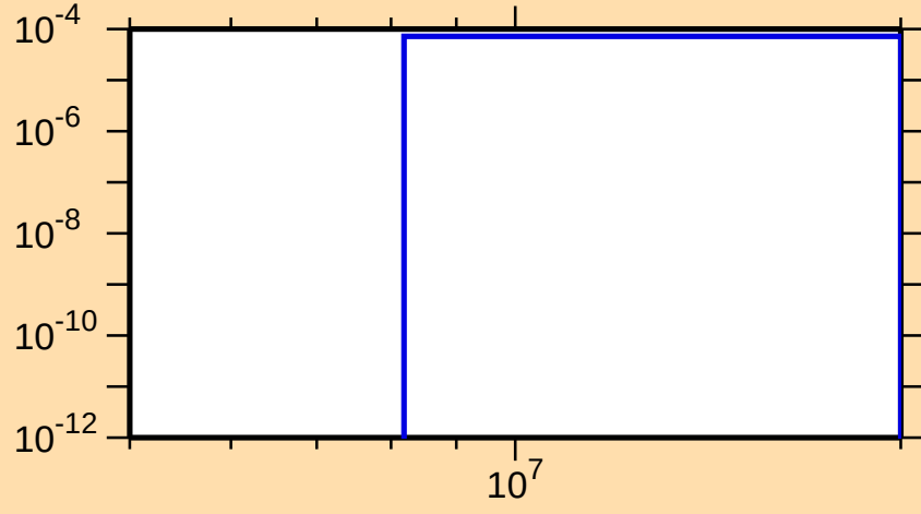
\sigma vs. E for ^{223}\text{Bi}(n,p)
