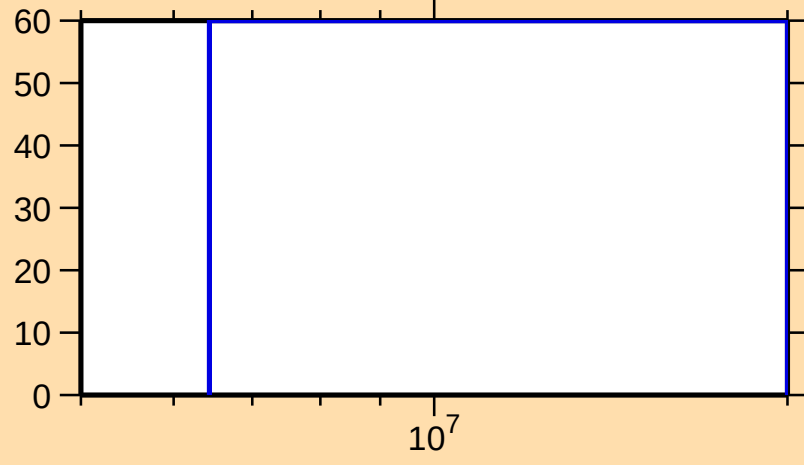
\Delta\sigma/\sigma vs. E for ^{223}\text{Bi}(n,n\text{cont.})
