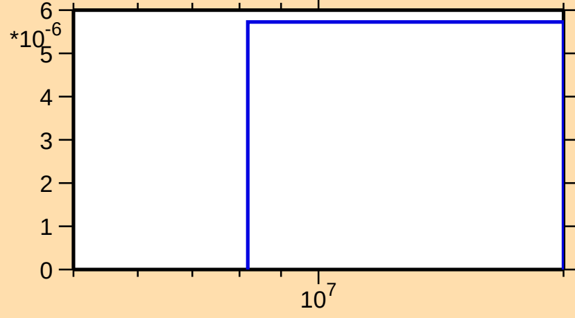
\sigma vs. E for ^{223}\text{Bi}(n,d)
