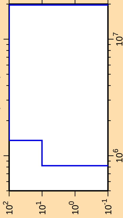
\Delta\sigma/\sigma vs. E for ^{70}\text{Br}(n,\text{He}3)
