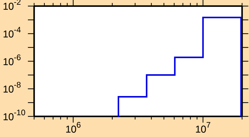
\sigma vs. E for ^{70}\text{Br}(n,\text{He}3)
