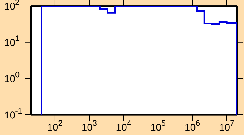
\Delta\sigma/\sigma vs. E for ^{70}\text{Br}(n,n_1)
