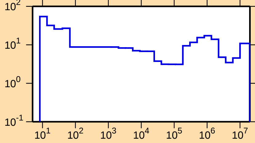
\Delta\sigma/\sigma vs. E for ^{70}\text{Br}(n,\text{el.})
