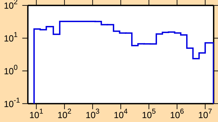
\Delta\sigma/\sigma vs. E for ^{70}\text{Br}(n,\text{tot.})
