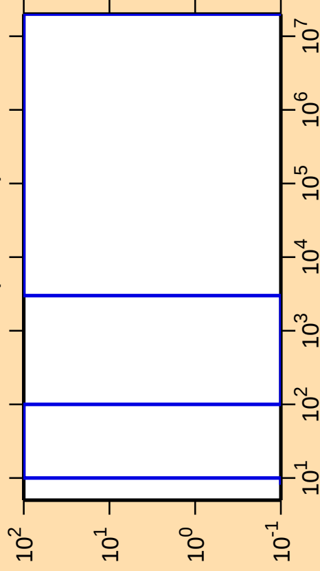
\Delta\sigma/\sigma vs. E for ^{70}\text{Br}(n,\text{ncont.})
