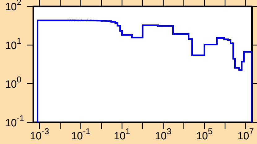
\Delta\sigma/\sigma vs. E for ^{70}\text{Br}(n,\text{tot.})
