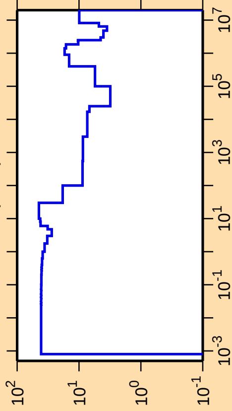
\Delta\sigma/\sigma vs. E for ^{70}\text{Br}(n,\text{el.})
